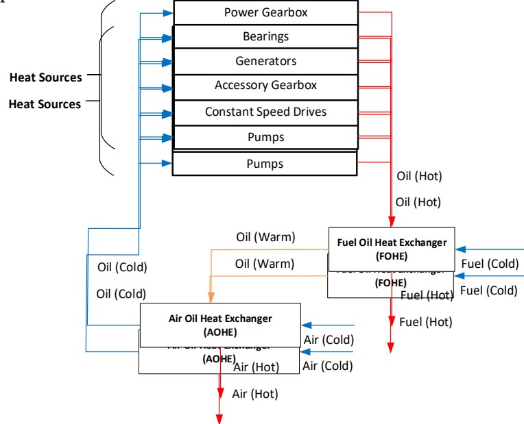
Figure 1. A conventional TMS architecture for aircraft applications (adapted from [6]).
