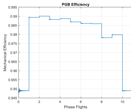
Figure 10. PGB mechanical efficiency during flight.
