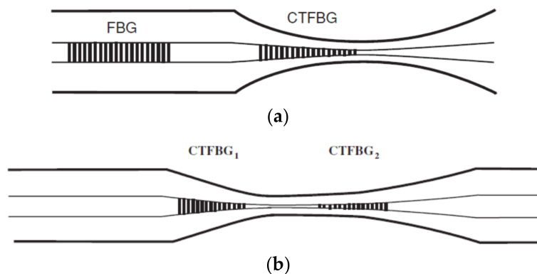
Figure 26. (a) Sensing head geometry with FBG/chirped tapered FBG (CTFBG) structure; and (b) sensing head geometry using two CTFBGs in biconical taper structure [155]. © IOP Publishing. Reproduced by permission of IOP Publishing. All rights reserved).
