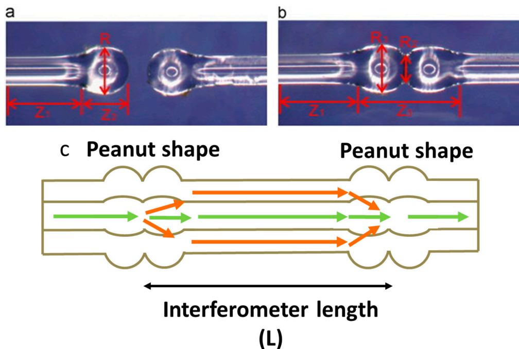
Figure 28. Microscopic image of the peanut-shape structure: (a) after the arc discharge treatment and (b) after the fusion splicing. Z_1 , distance to ellipsoidal-structure section Z_2 , length of ellipsoidal-structure section; R , radius of the ellipsoidal-structure section; (c) schematic diagram of the cascading two waist enlarged structures-MZI (adapted from [157]).
