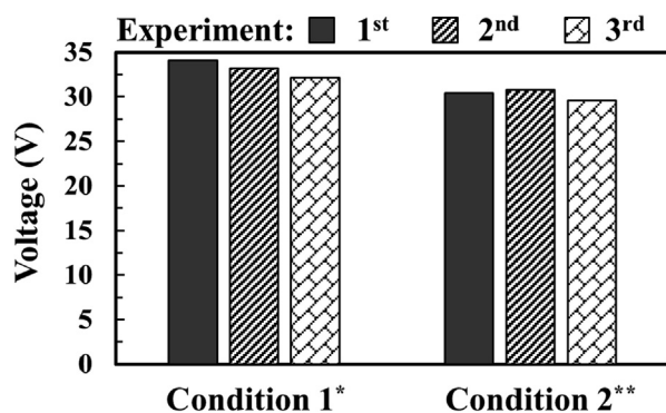
Fig. 4. Comparison of SOFC stack performance over three successive experiments and after formation of localised burnt zone. *Condition 1: Representing the stack OCV at hydrogen and air flow rates of 4 and 12 L min -1 , respectively. **Condition 2: Representing the stack voltage at stack current of 8 A, and hydrogen and air flow rates of ~35 and 116 L min -1 , respectively.
