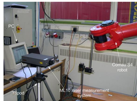
Fig. 5 Experimental setup for robot accuracy measurements
