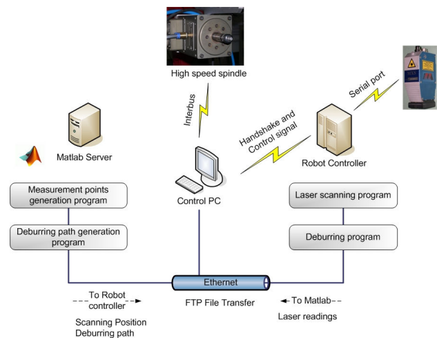
Fig. 3 Cell control architecture
