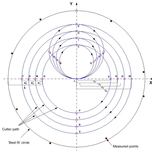
Fig. 1 Schematic diagram of cutting path generation
