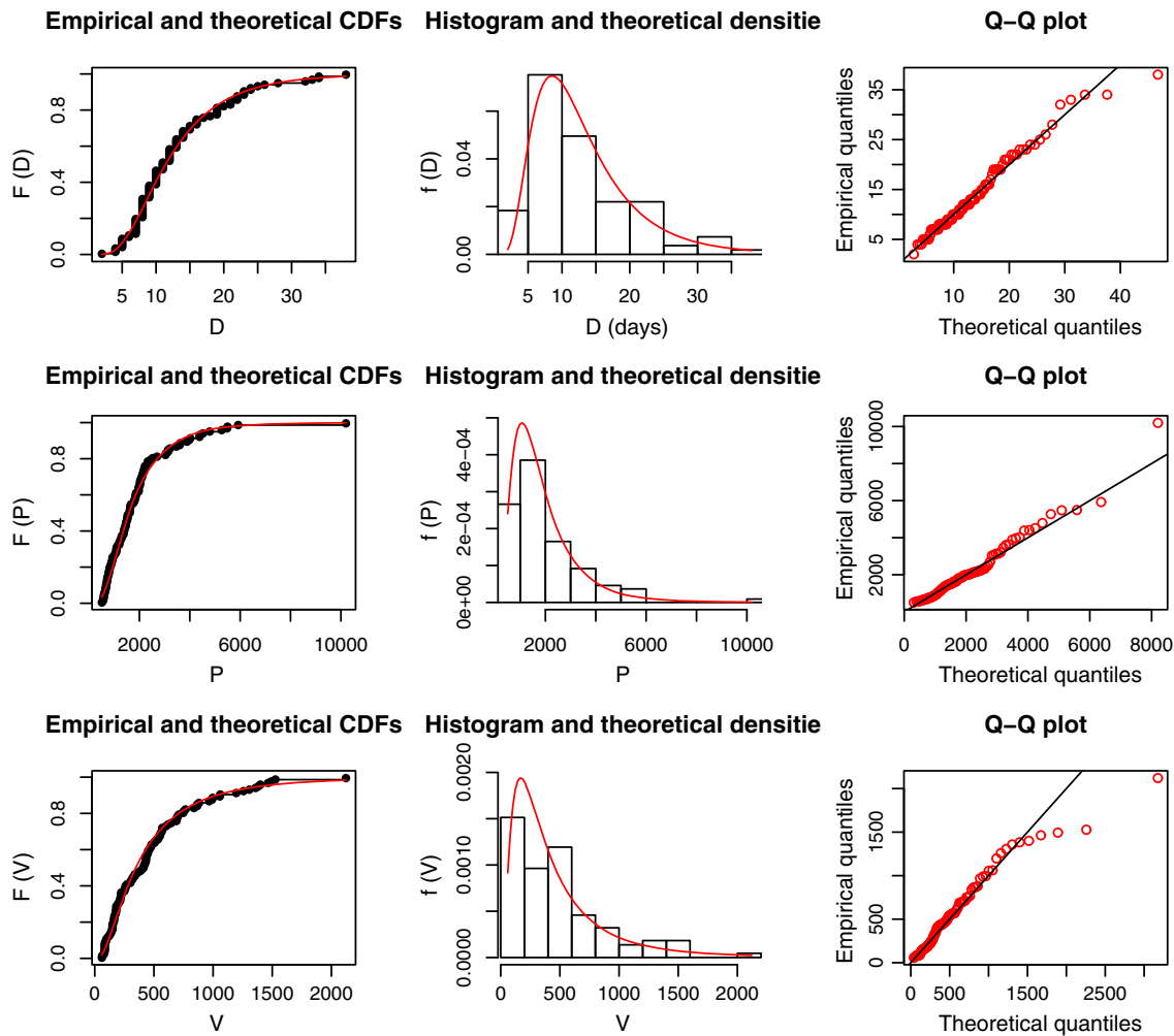
Fig. 4. Fitted distributions to the flood variables D, P, V , are respectively shown in the 1st to 3rd rows. The 1st to 3rd columns illustrate cdf, pdfs and q-q plots of the flood variables, respectively.
