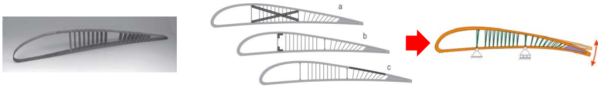
Figure 3: Belt-Rib concept showing demonstrator (left), activation (centre) and deformation (right) [31]
