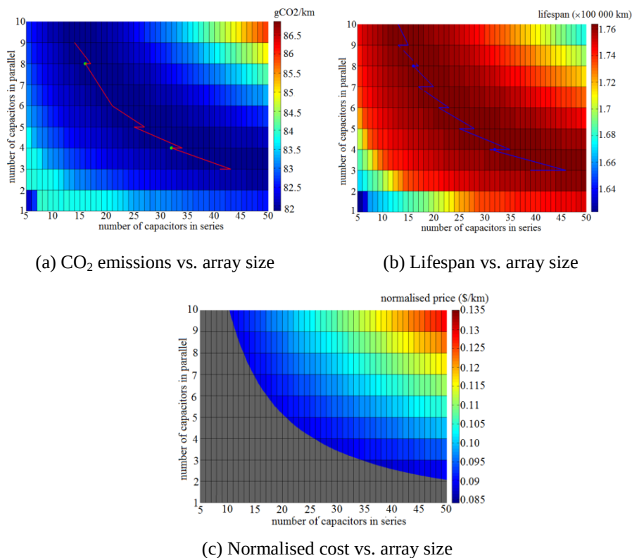
Figure 5. Variation of vehicle performance measures with super capacitor array size
