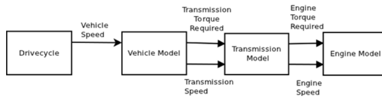
Figure 1. Backward-facing model
