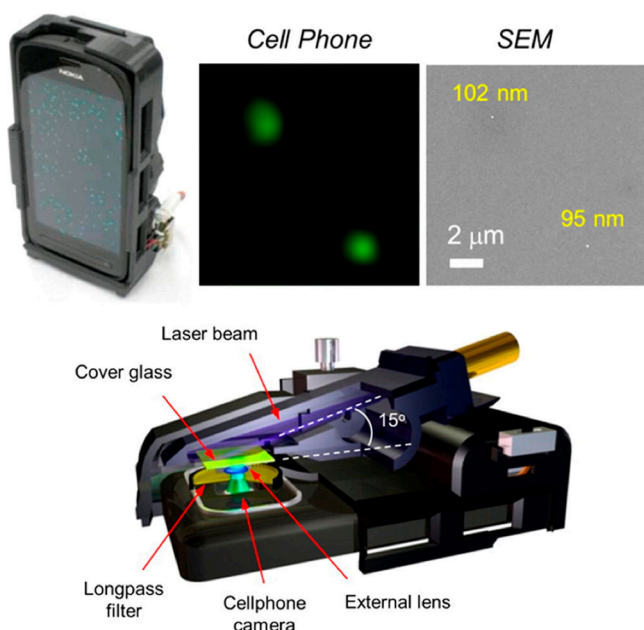
Figure 8. Imaging single viruses using a smartphone. A smartphone-based optomechanical attachment with a resolution of <50 nm for the detection of individual viruses. Reprinted with permission from ref 170. Copyright 2013 American Chemical Society.
