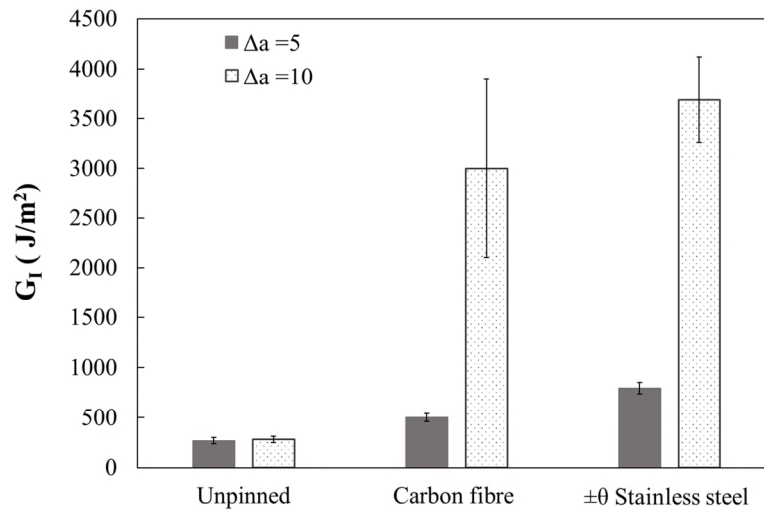
Figure 10 Average apparent G_I at \Delta a = 5 mm and \Delta a = 10 mm. ( Mode I DCB test )
