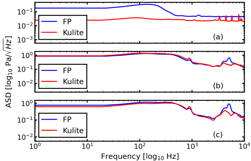
Figure 10. Amplitude spectral density (ASD) determined from the FP and Kulite pressure sensors acquiring at 24 kHz and 20 kHz, respectively, for no wind speed (a) and during the 18^\circ (b) and 20^\circ (c) AOA steady-state runs at a wind speed of 40 \text{ m s}^{-1} .
