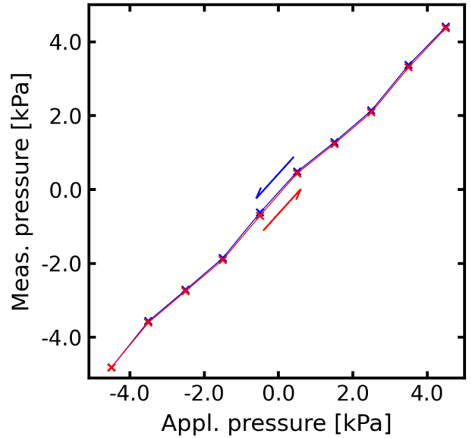
Figure 6. The response of the FP pressure sensor following the application of a pressure cycle from 4.5 \text{ kPa} to -4.5 \text{ kPa} then returning to 4.5 \text{ kPa} , where the blue and red arrows indicate decreasing and increasing pressure, respectively.
