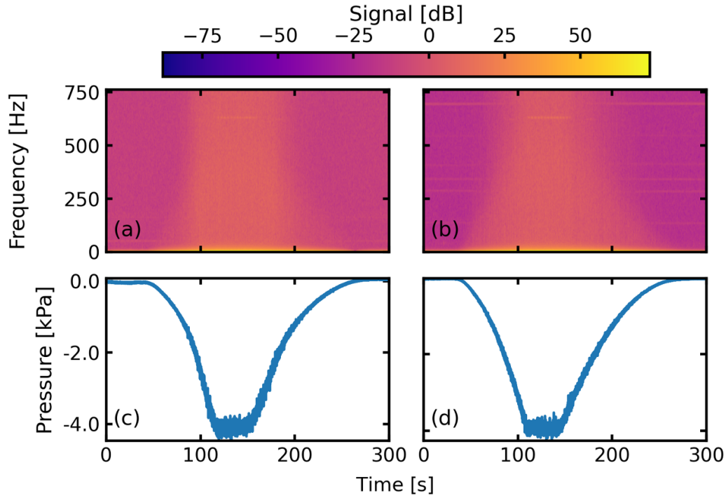
Figure 9. Spectrograms for FP (a) and Kulite (b) pressure sensors during the ramped wind speed protocol at 20^\circ AOA with their associated time series (c) and (d), respectively.
