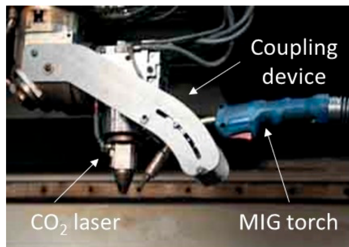
Figure 5. Laser-MIG coupling.
