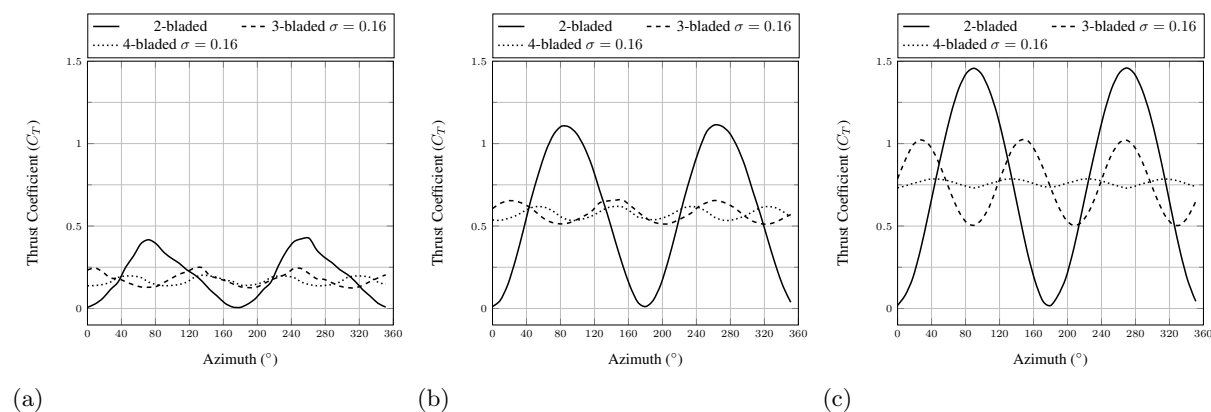
Figure 5. Instantaneous thrust coefficient at \text{TSR} = 2.02 (a), \text{TSR} = 4.6 (b) and \text{TSR} = 7.98 (c).
