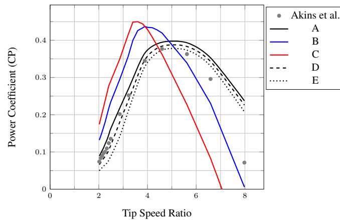
Figure 3. Power curves for five different turbine models.
