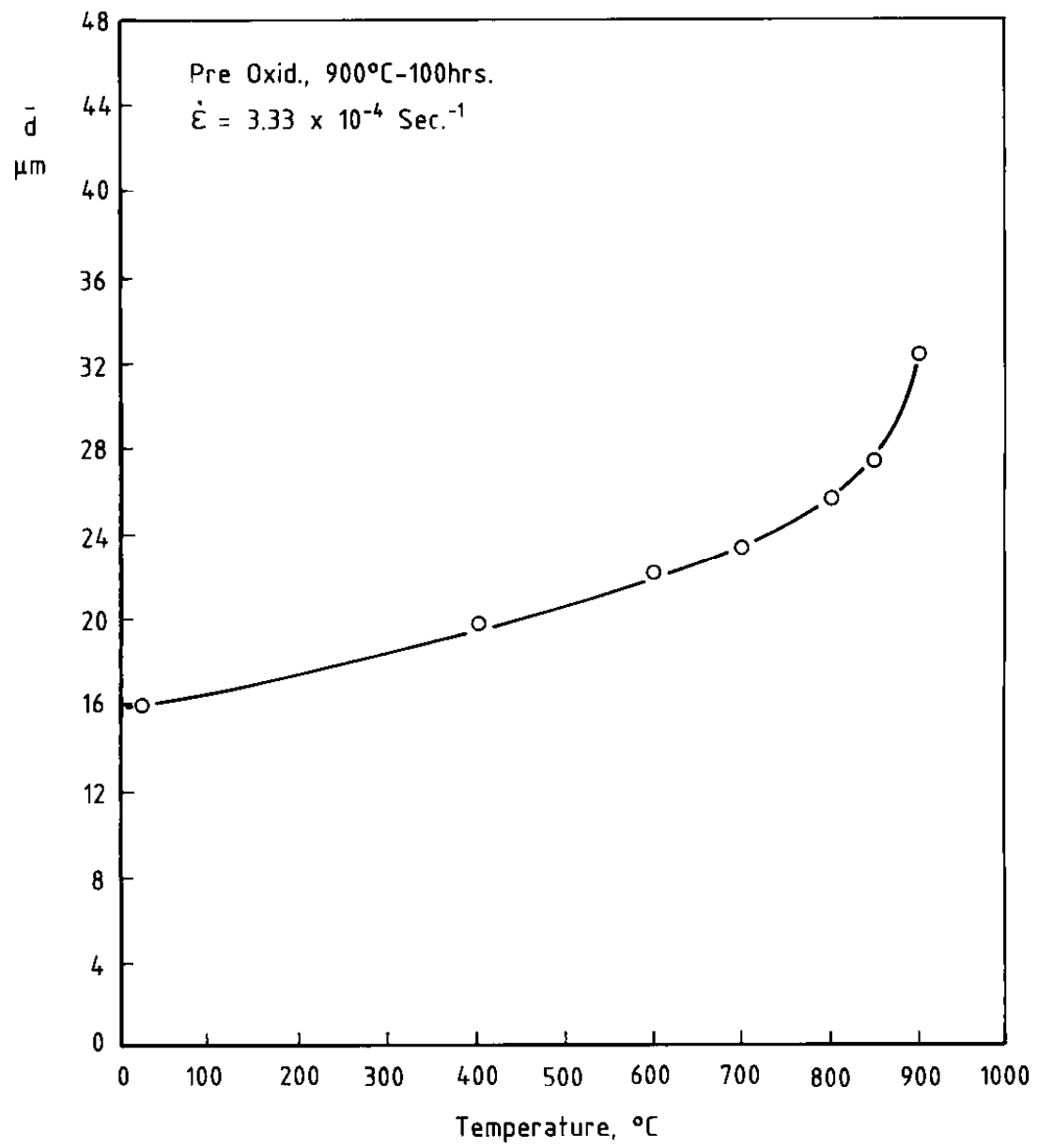
Figure 3 Characteristic crack separation \bar{d} as a function of temperature in the strain rate independent region.
