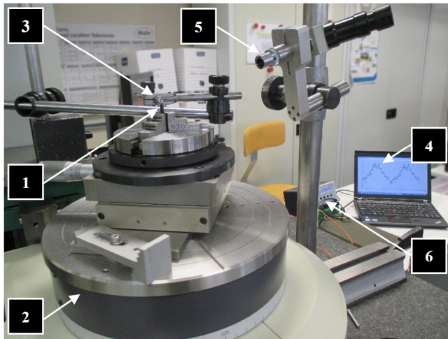
Figure 1. The sample (1) is held by the chuck on the rotary table (2), while the chromatic confocal sensor (3) is observing its surface. On the computer screen (4), the acquisition can be seen. Behind the holder of the magnifying lens used for pre-alignment (5), the controller (6) displays the distance in real time.
