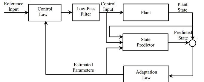
Fig. 3. The \mathcal{L}_1 adaptive controller.
