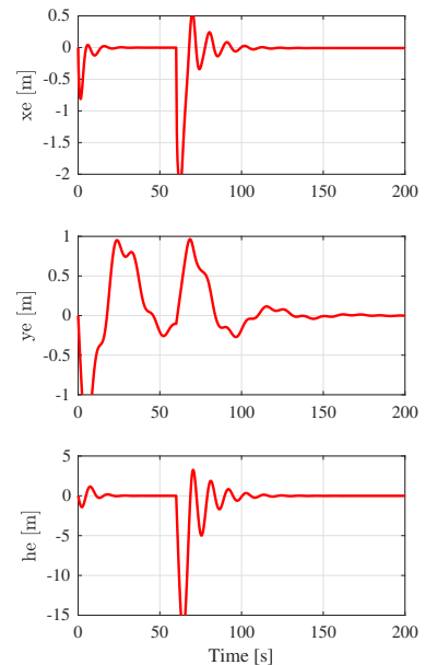
(b) Trajectories errors
