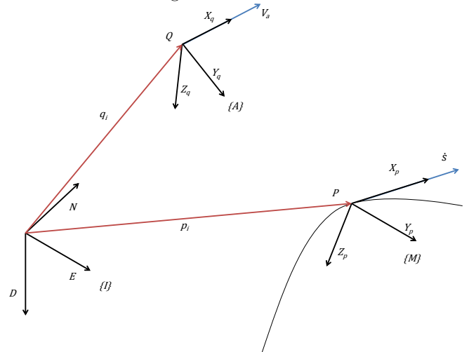
Fig. 1. Curved Path-Following Frames.
