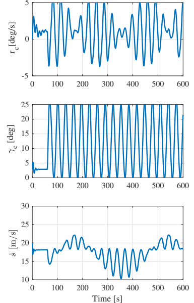
(a) Output commands \mathcal{L}_1 adaptive controller.
