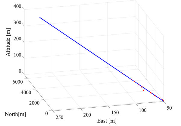
(a) Airship 3D trajectory (Desired blue).
