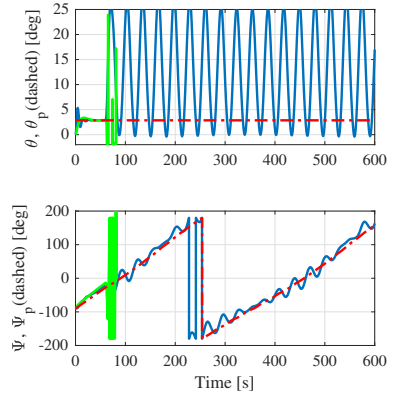
(b) Trajectories errors ( \mathcal{L}_1 blue, AIB green).
