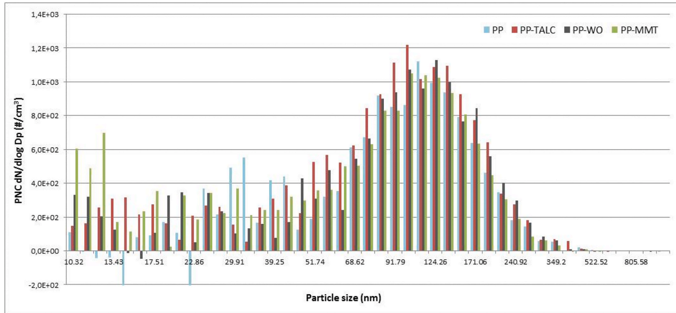
Fig. 3. Average of PSD at peak concentration expressed as dN/d\log D_p \, (\#/cm^3) having subtracted background concentration corresponding to airborne particle release measurements using the protocol to simulate an industrial drilling process (SMPS + C Data) for PP; PP-Talc; PP-WO and PP-MMT samples.
