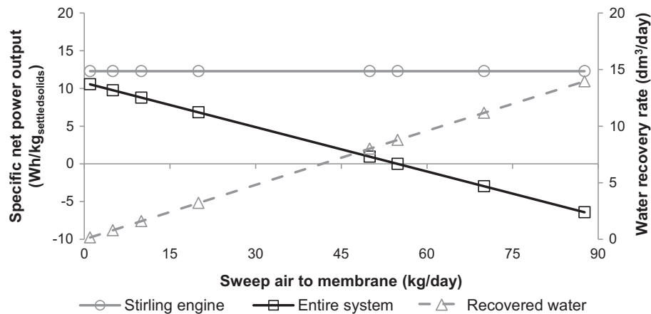
Fig. 5. Effect of the amount of sweep air fed to membrane on specific power output and water recovery rate.
