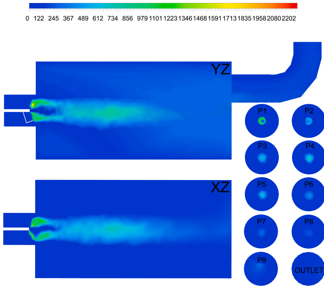
Fig. 8. \text{NO}_x emission [ppm] of the ammonia combustion in the boiler at YZ and XZ Planes, and 9 planes perpendicular to the air and fuel flow with a distance increment of 10 cm from the outlet plane.
