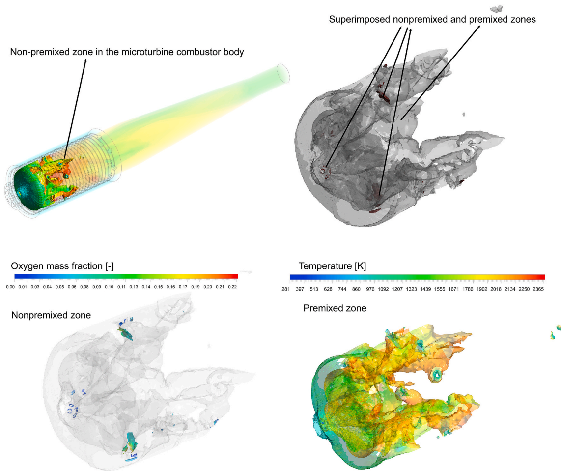
Fig. 15. Nonpremix and premix zones in the gas turbine combustor isosurfaces coloured by oxygen concentration and temperature.
