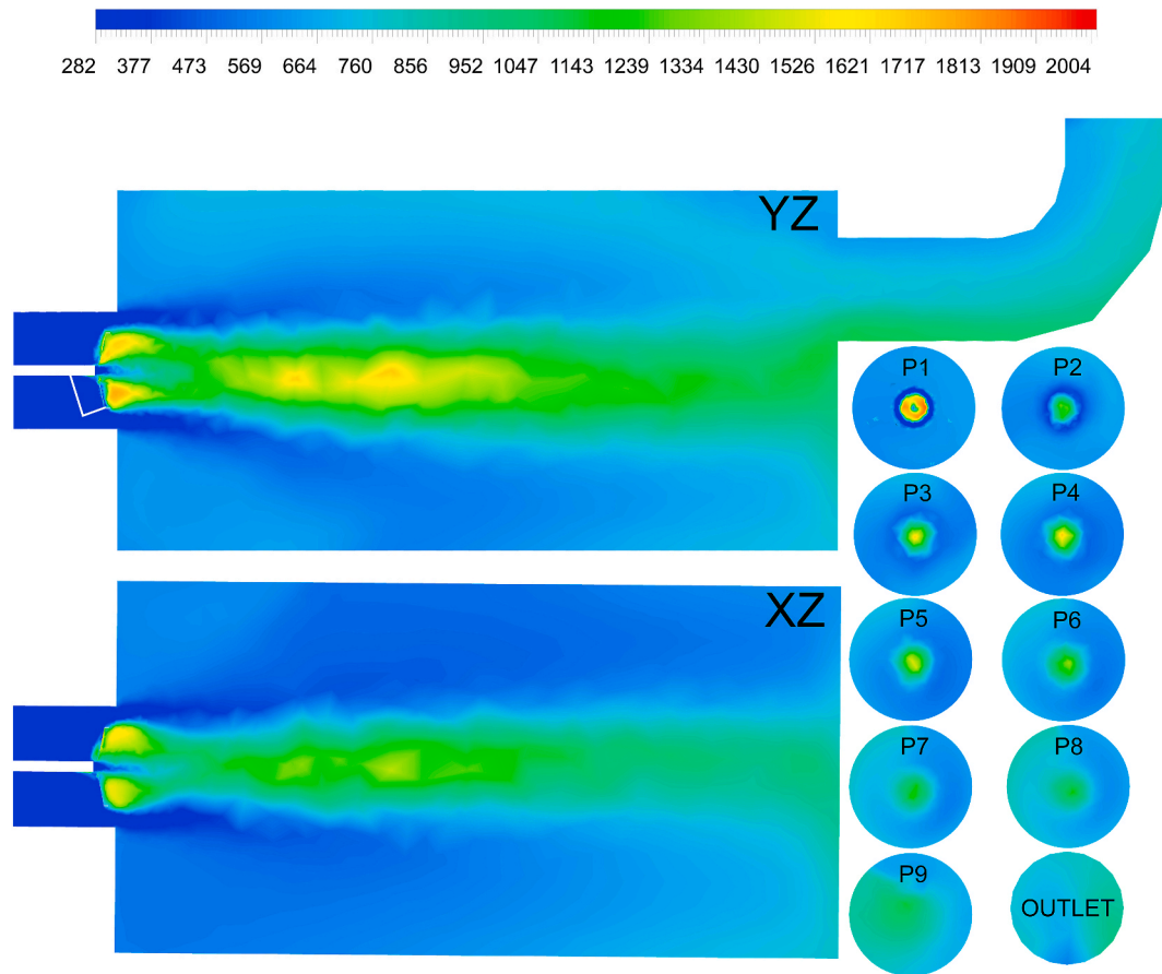
Fig. 6. Temperature contour [K] of the ammonia combustion in the boiler at YZ and XZ Planes, and 9 planes perpendicular to the air and fuel flow with a distance increment of 10 cm from the outlet plane.
