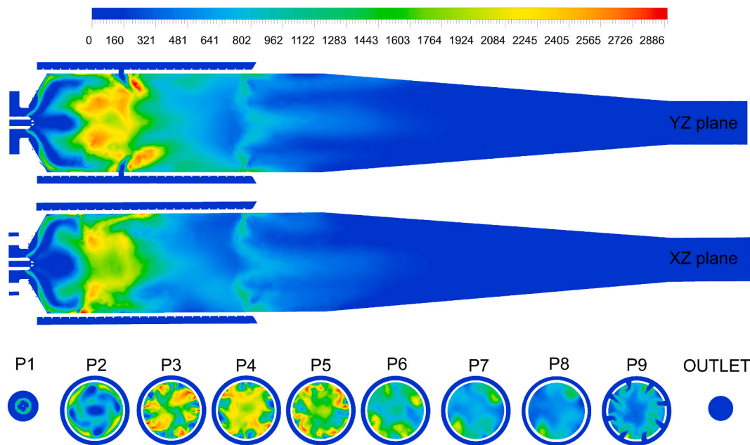
Fig. 13. \text{NO}_x emissions [ppm] of the ammonia combustion in the turbine at YZ and XZ Planes, and 9 planes perpendicular to the air and fuel flow with a distance increment of 2 cm from the outlet plane.
