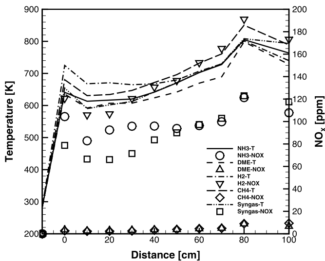
Fig. 9. The temperature and \text{NO}_x emissions averaged on the perpendicular planes along with the flow in the boiler for ammonia, DME, hydrogen, methane and syngas.
