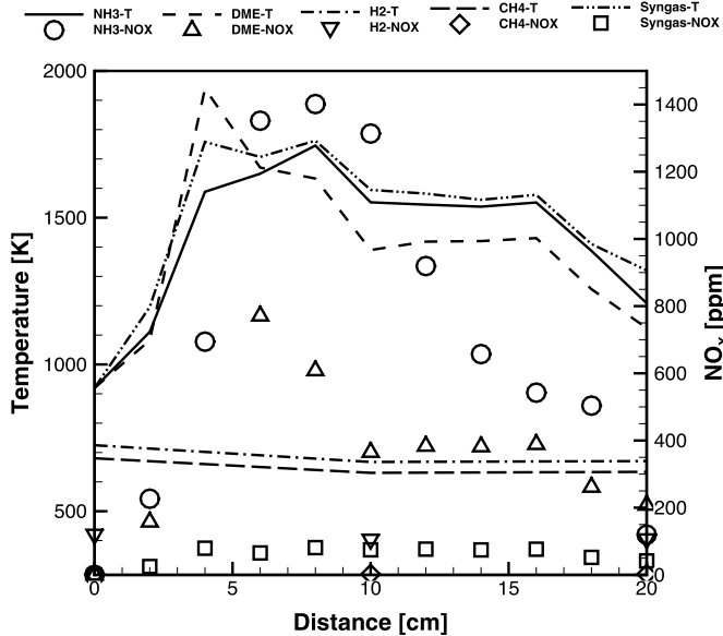
Fig. 14. The temperature and \text{NO}_x emissions, averaged on the perpendicular planes, along with the flow in the turbine for ammonia, DME, hydrogen, methane and syngas.
