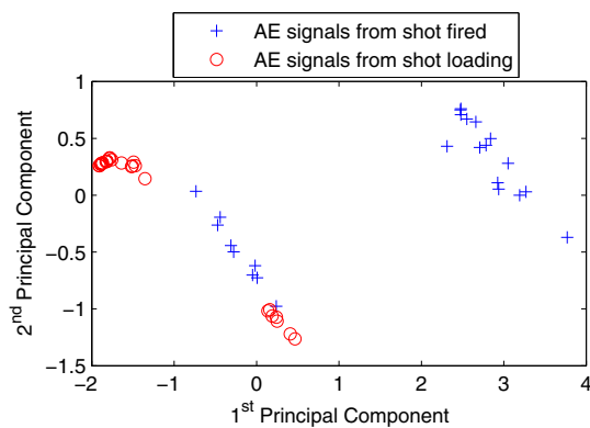
Fig. 6. PCA of AE signals detected from shot rounds fired and loading/unloading mechanism at Sensor 1 located on the rifle butt
