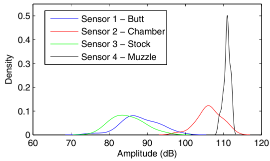
Fig. 4. Amplitude distribution of AE signals detected by the sensors at various locations from shot rounds fired
