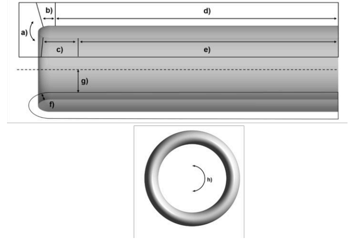
Figure 6: Grid blocks refined in the sensitivity analysis across the various parts of the intake duct. Grid blocks indicated in lower case letters.
