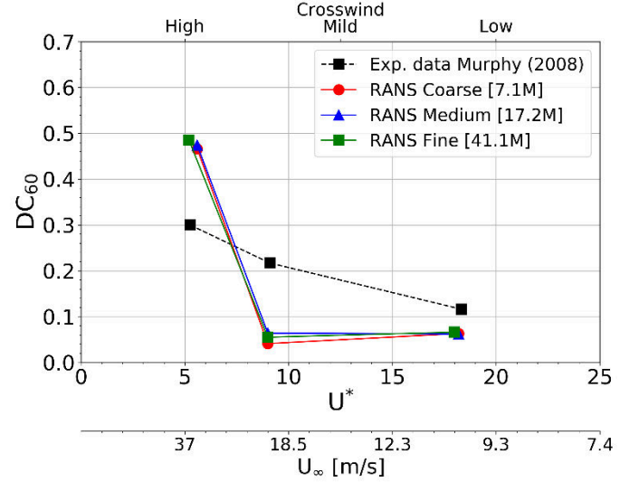
Figure 10: Fan face distortion across the range of U^* for three computational grids and experimental data.
