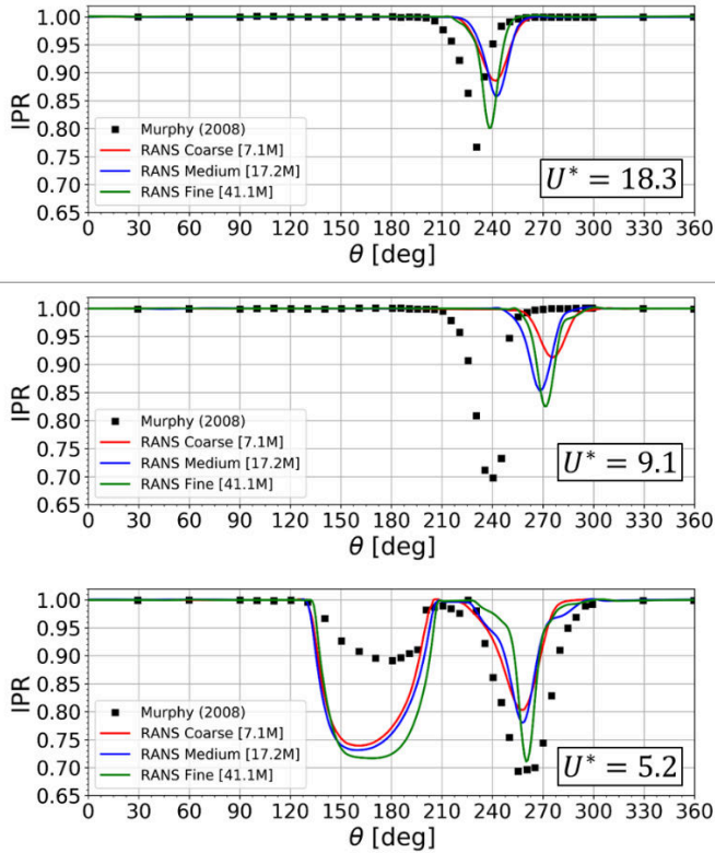
Figure 9: Numerical and experimental azimuthal loss distributions at a fixed radial position crossing the peak loss flow regime across the range of U^* and grid resolutions. Experimental data points derived from Figure 7.
