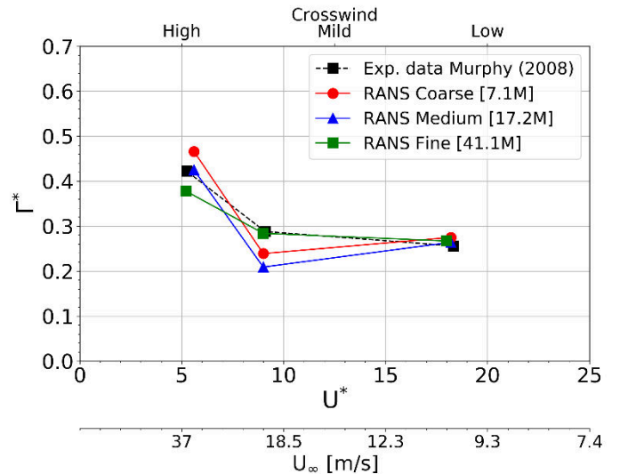
Figure 11: Ground vortex non-dimensional circulation across the range of U^* for three computational grids and experimental data.
