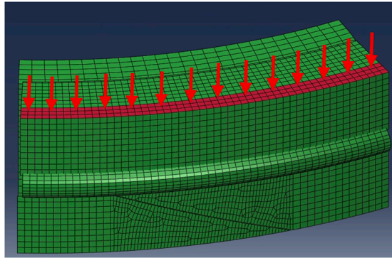
Fig. 8. Seal Pack: Region of uniform 20 MPa applied pressure.
