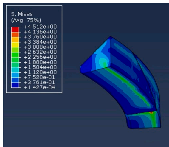
Fig. 27. Interference fit stress levels.
