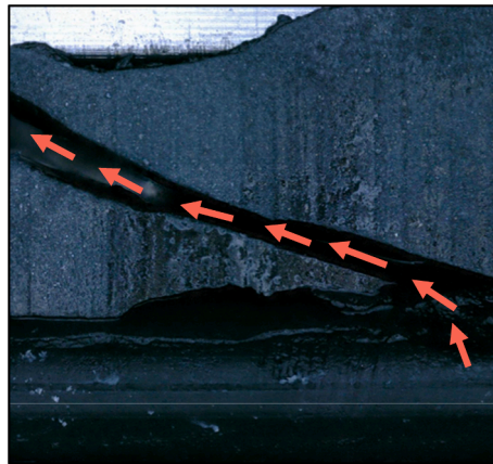
Fig. 16. Fluid flow through back-up ring gap.
