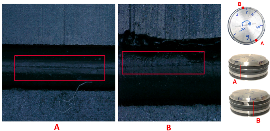
Fig. 15. Pre-extrusion elastomer thermal degradation.
