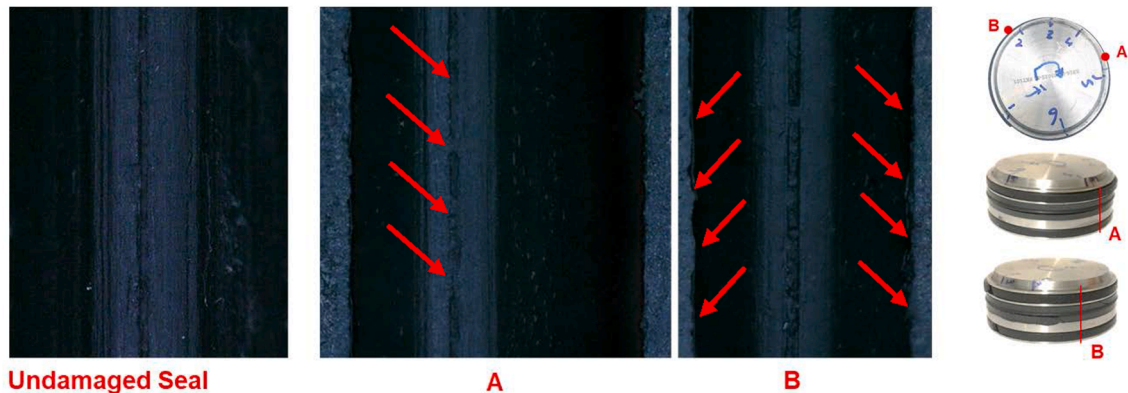
Fig. 13. Flash line wear and thermal degradation.
