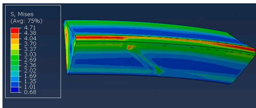
Fig. 30. Pressure step: elastomer stress levels.
