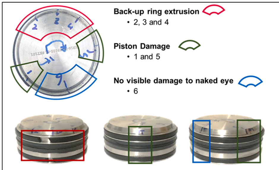
Fig. 4. Overview of sections of interest for on failed sample.
