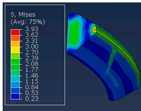
Fig. 29. Temperature step: elastomer stress levels.
