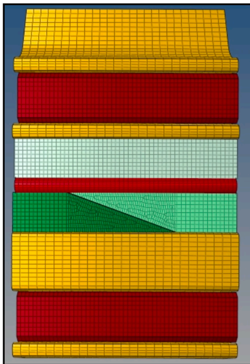
Fig. 6. Meshed piston and sealing components.
