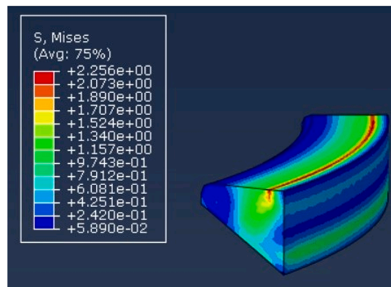
Fig. 28. Interference fit: seal pack stress levels.
