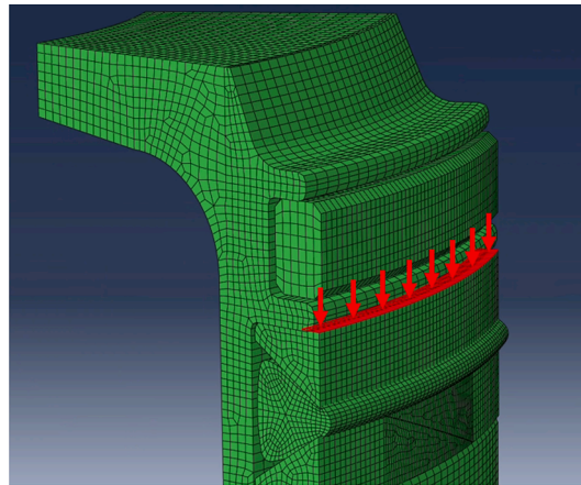
Fig. 9. Seal pack and piston assembly: Region of uniform 20 MPa applied pressure.
