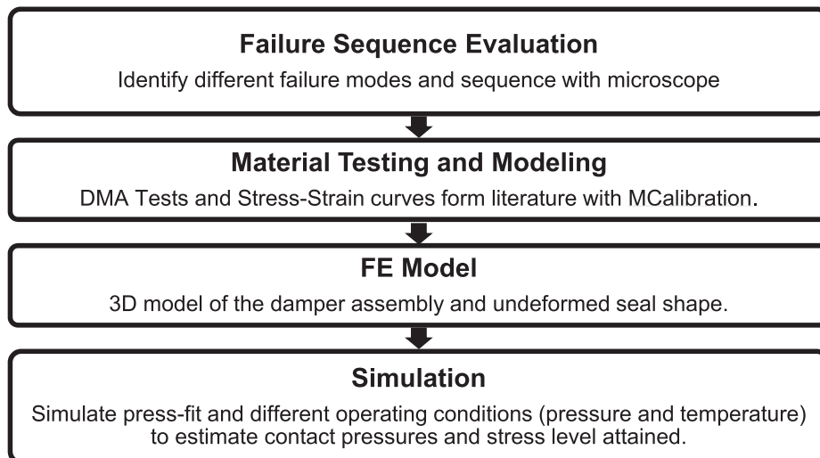
Fig. 3. Steps adopted in the methodology.
