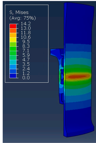
Fig. 23. Interference fit stress levels.
