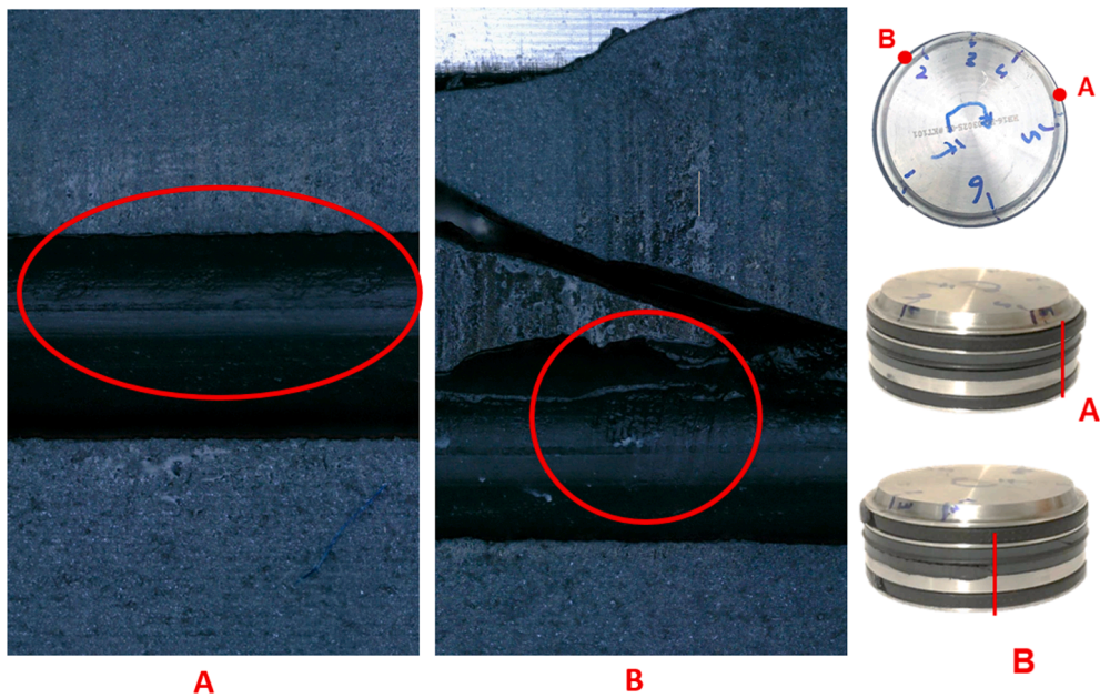
Fig. 14. Pre-Extrusion elastomer nibbled extrusion.
