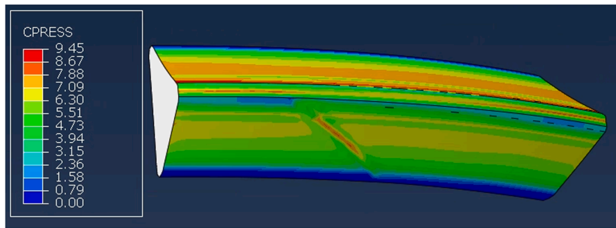
Fig. 31. Pressure step: elastomer contact stress.
