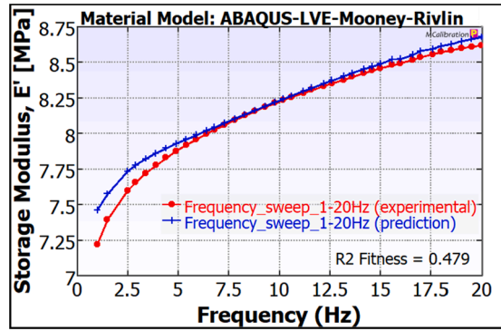
Fig. 22. Fluorocarbon DMA Data fitted with Mooney-Rivlin Model.
