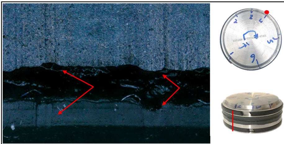
Fig. 10. Elastomer and low-pressure back-up ring wear alignment – section 4.
