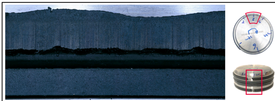
Fig. 18. Section 3 PTFE extrusion.
