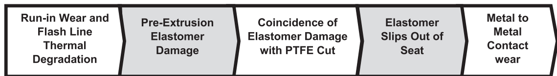
Fig. 12. 5-step failure sequence summary.
