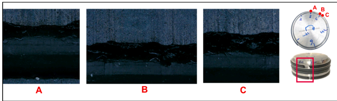
Fig. 19. Unseating damage to the elastomer.
