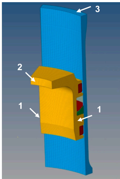
Fig. 7. Cut 3D FE Model.
