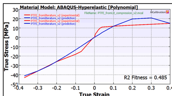
Fig. 21. PTFE stress-strain curve fitted with a hyperelastic polynomial model.
