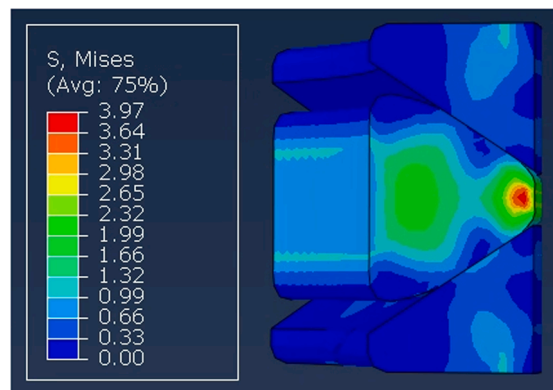
Fig. 24. Interference fit: seal pack stress levels.
