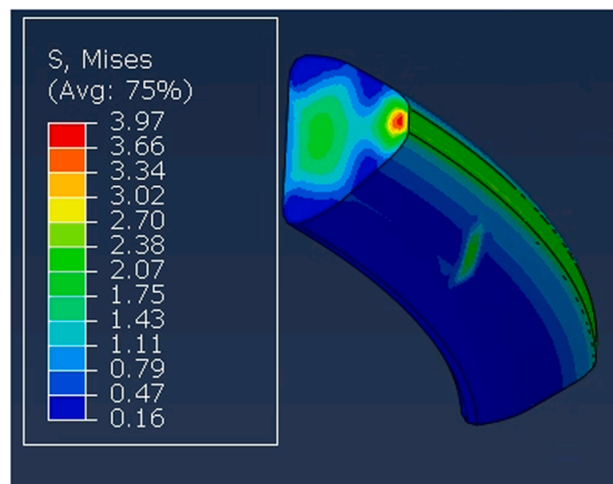
Fig. 25. Elastomer stress levels.
