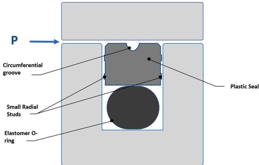
Fig. 32. Suitable seal example.
