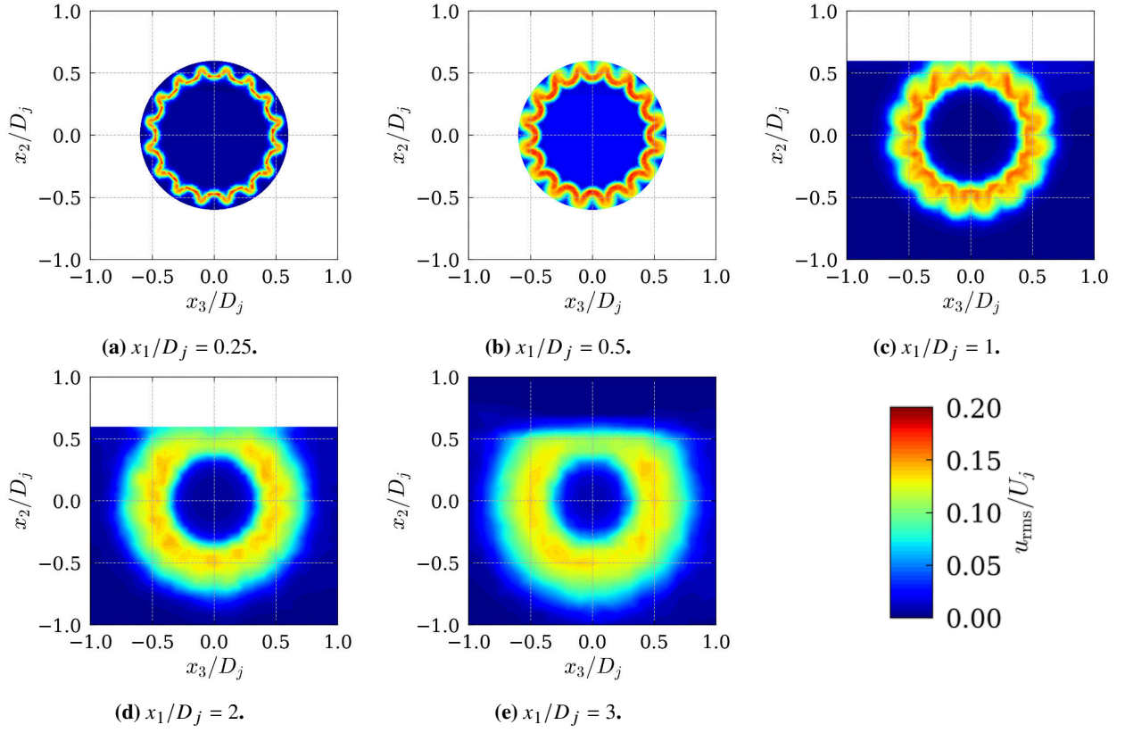
Fig. 9 RMS of the axial velocity at several planes downstream of the nozzle exit obtained with the simulation denoted Chevron-1 in Table 2. For the first two planes, only a limited radial extent of the flow was sampled.
