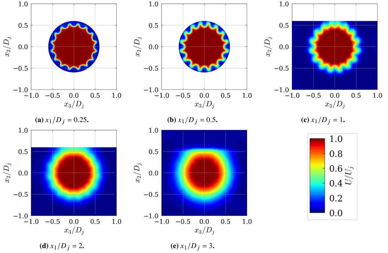
Fig. 7 Mean axial velocity at several planes downstream of the nozzle exit obtained with the simulation denoted Chevron-1 in Table 2. For the first two planes, only a limited radial extent of the flow was sampled.
