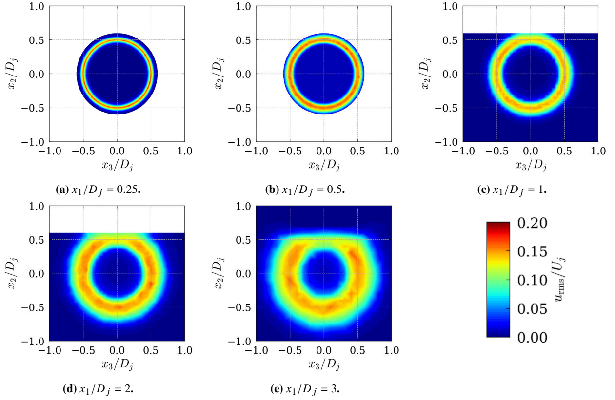
Fig. 8 RMS of the axial velocity at several planes downstream of the nozzle exit obtained with the simulation denoted Installed-1 in Table 2. For the first two planes, only a limited radial extent of the flow was sampled.
