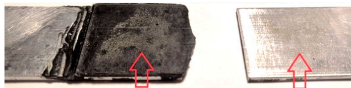
Figure 17. Ultimate adhesion failure in single-lap bonded joint specimen (arrows point bonded areas).
