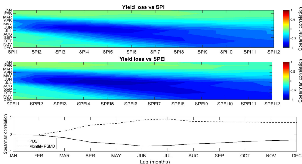
Fig. 7. Heat maps showing the Spearman's Rank correlation coefficient ( \rho ) between monthly SPI and SPEI and Sirius simulated wheat yield loss at Cambridge (1912-2015). Also shown are the monthly correlations between yield and PSMD and PDSI.
