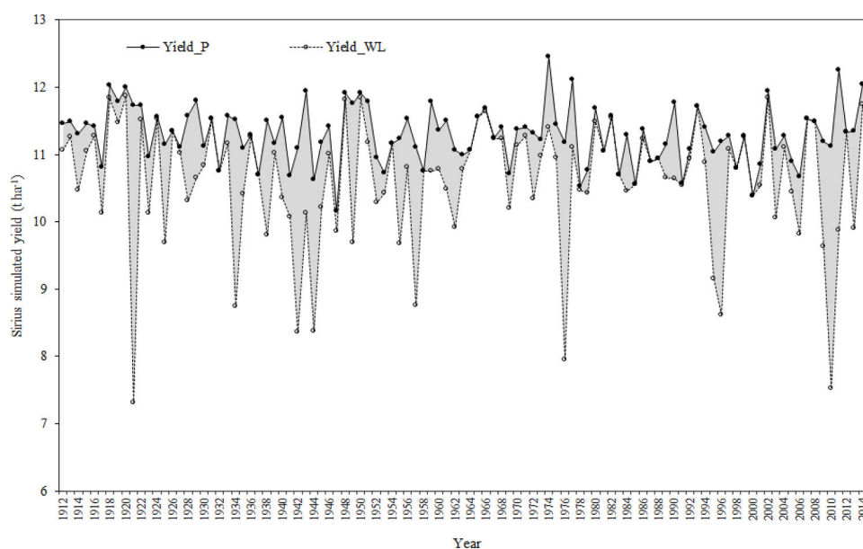
Fig. 6. Sirius simulated annual potential (Yield_P) and water limited (Yield_WL) wheat yield ( \text{t ha}^{-1} ) between 1912 and 2015.
