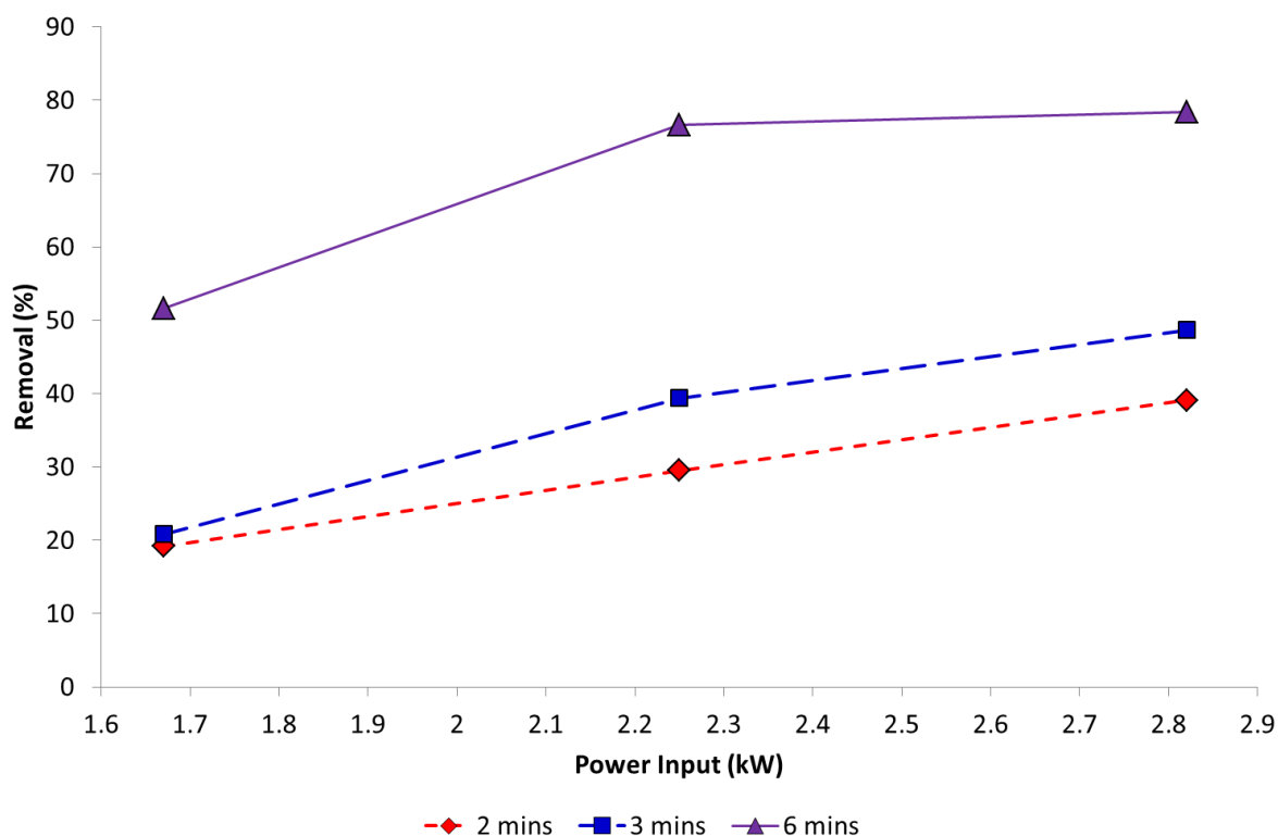
Figure 6. Influence of residence time on the degradation of metaldehyde in MF permeate as a function of power input, 16 \text{ mg L}^{-1} \text{ H}_2\text{O}_2 .
