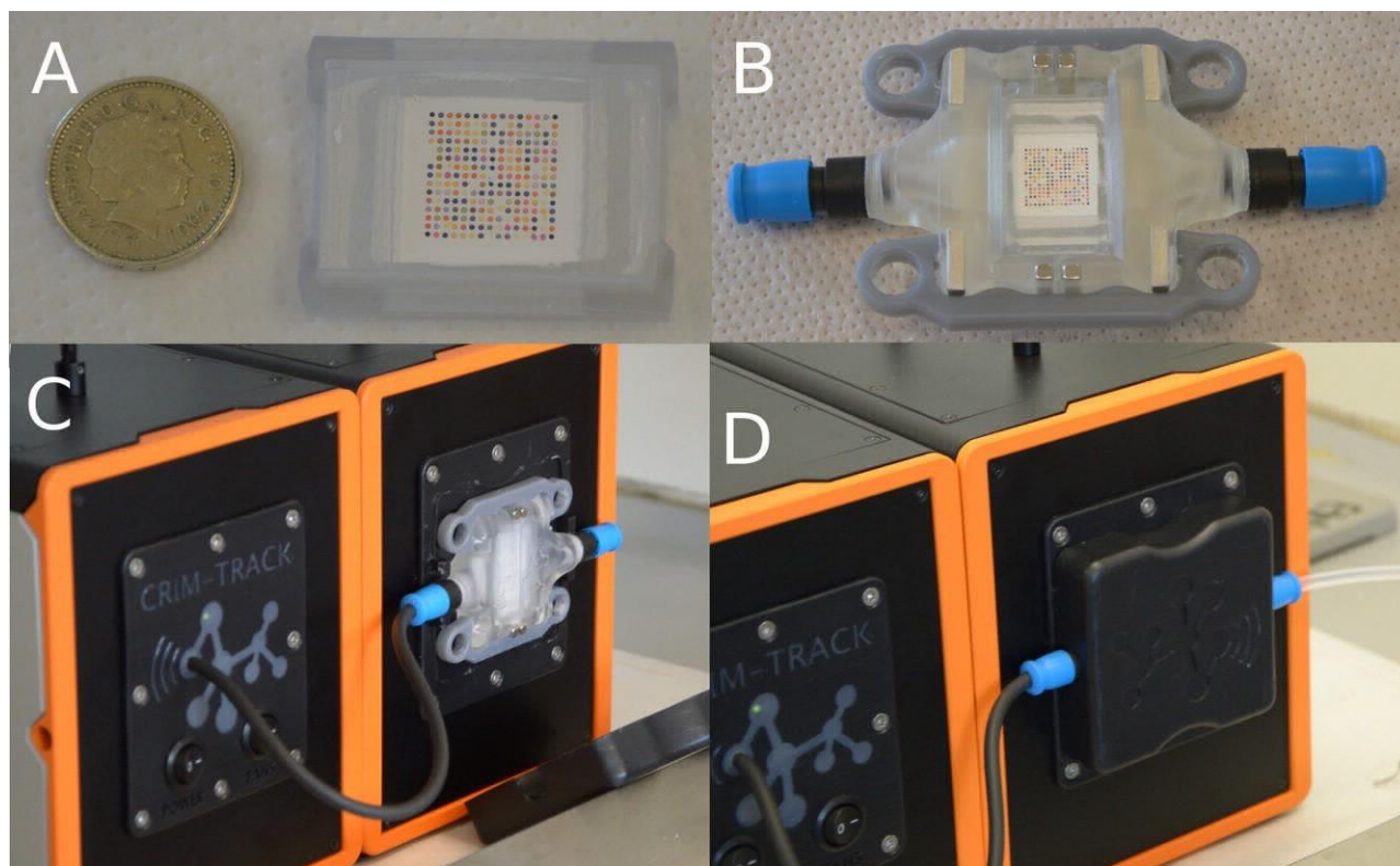
Figure 2: Mounting sensor chip in current prototype. A: Chip in rubber chip carrier, £1 coin as size reference. B: Chip loaded into flow chamber, grey clamps ensure air tightness. C: Flow chamber clicked into place on prototype, black downstream air tubing connected. D: Black light blocking hood mounted atop flow chamber, clear upstream air sample tubing connected.
