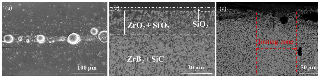
Fig. 14 Microstructures after oxidation at 1200 °C for 1 h: (a) surface of ZS/Ni/ZS joint, (b) and (c) cross-sectional morphologies of the base \text{ZrB}_2\text{-SiC} ceramics and joining zone.
