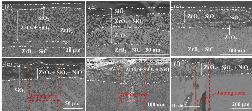
Fig. 16 Cross-sectional morphologies after oxidation at 1600 °C: (a)-(c) base \text{ZrB}_2 -SiC ceramics oxidised for 0.5, 1 and 2 h, respectively; (d)-(f) joining zone oxidised for 0.5, 1 and 2 h, respectively.
