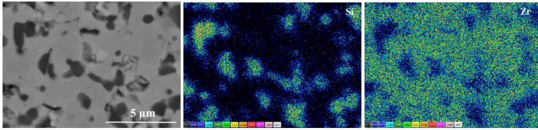
Fig. 6 Microstructure and chemical element distributions in the base \text{ZrB}_2\text{-SiC} ceramics.
