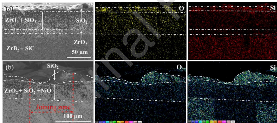
Fig. 15 Cross-sectional morphologies and distribution maps of chemical elements after oxidation at 1400 °C for 1 h: (a) base \text{ZrB}_2\text{-SiC} ceramics and (b) joining zone.
