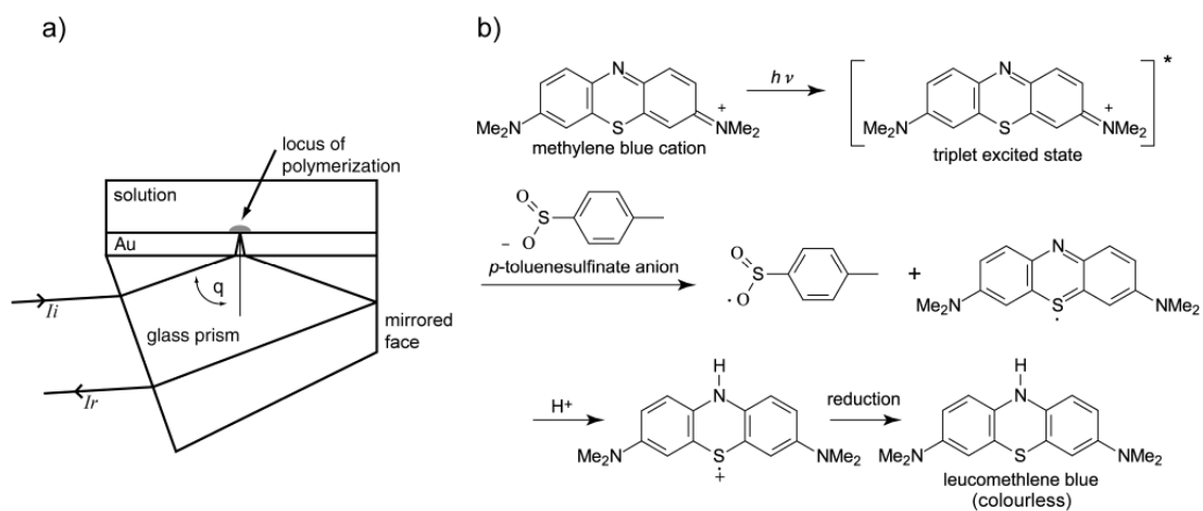
Figure 1. a) Schematic of the SPR optical prism configuration used, b) Scheme showing the photoreduction of the triplet excited state of methylene blue and formation of the bleached form of the dye, leucomethylene blue. It is likely that radicals derived from the p -toluenesulfinate radical are the active initiating species (Margerum et al. , 1971).
