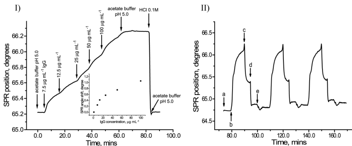
Figure 6. I) The SPR response for the protein G-modified cross-linked poly(MAA) matrix in response to the addition of increasing concentrations of IgG (in acetate buffer, pH 5.0). Inset: The same data represented in isotherm format; II) Reproducibility of the sensor response using protein G-modified cross-linked poly(MAA) film over three cycles. The arrows mark the addition of the following solutions: a) acetate buffer pH 5.0; b) 100 \mu\text{g mL}^{-1} IgG in acetate buffer, pH 5.0; c) acetate buffer pH 5.0; d) 0.1M HCl and e) acetate buffer pH 5.0.
