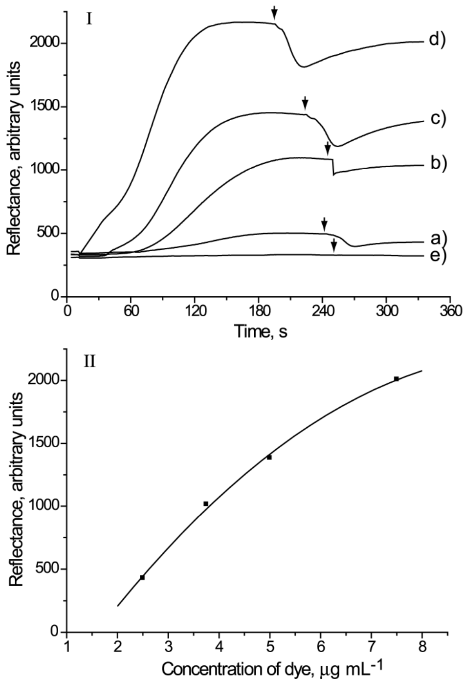
Figure 3. I) Time course of polymerization followed by monitoring the reflectance intensity for varying concentrations of methylene blue: a) 2.5; b) 3.75; c) 5; d) 7.5 \mu\text{g mL}^{-1} and e) control experiment performed in the absence of dye. The arrows indicate the time when the flow cell was flushed with clean water. II) Relationship between concentration of
