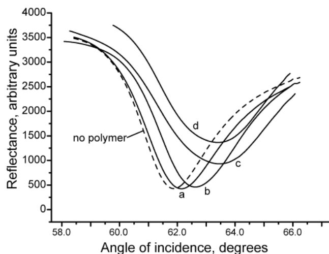
Figure 4. SPR curves corresponding to the conditions used in Figure 3-I (curves a-d), the curve for bare gold (dashed line) was recorded with water alone in the flow cell, the curves a-d were recorded for water-filled cells following polymerization, the displacement of the SPR curve being due to the presence of thin polymer layers attached to the gold surface. Dye concentrations used were as follows: a) 2.5 \mu\text{g mL}^{-1} ; b) 3.75 \mu\text{g mL}^{-1} ; c) 5.0 \mu\text{g mL}^{-1} ; d) 7.5 \mu\text{g mL}^{-1} . From an analysis of the SPR curves, the calculated refractive index of the polymer layers was estimated to be: real part: 1.345-1.348, imaginary part: 0.03-0.04. The calculated thickness of layers was: a) 20 \pm 5 \text{ nm} , b) 60 \pm 10 \text{ nm} , c) 150 \pm 20 \text{ nm} , d) 200 \pm 30 \text{ nm} .
