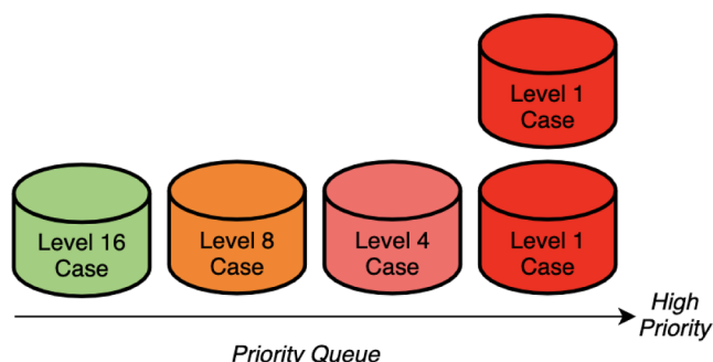
Fig. 2. A DFL priority queue formed by HiCaP allocation.
