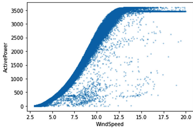
FIGURE 1 Wind turbine power curve correlation.
