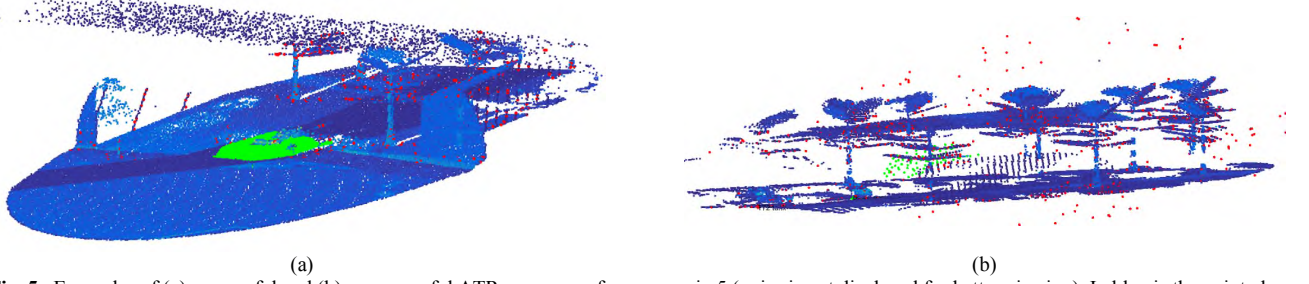
Fig. 5. Examples of (a) successful and (b) unsuccessful ATR on a scene from scenario 5 (noise is not displayed for better viewing). In blue is the point cloud scene, in red the remaining scene vertices after pre-processing and in green the transformed model template based on the Hypothesis generated
