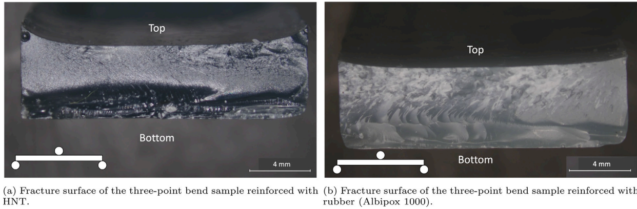
Fig. 16. Fracture surfaces of the selected three-point bend samples.
