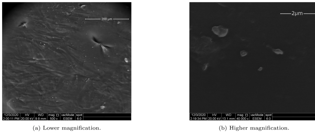
Fig. 8. EM images of an epoxy sample reinforced with rubber (seen as regions with lighter colour with diameter of approximately 0.5 – 1 μm).
