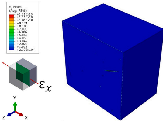
Fig. 22. A section view of an RVE with ellipsoidal HNT inclusions with diameters from 30 nm to 70 nm and lengths from 1 \mu\text{m} to 3 \mu\text{m} (Stress unit: GPa).
