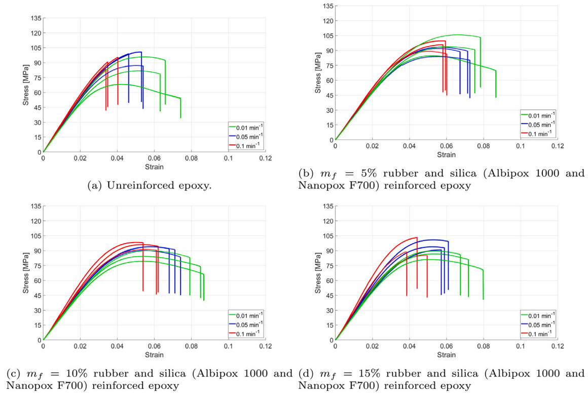
Fig. 15. Stress–strain curves of rubber and silica (Albipox 1000 and Nanopox F700) reinforced epoxy.
