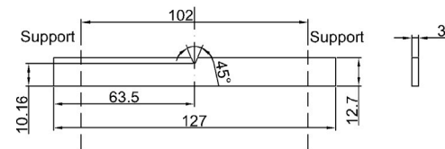
Fig. 3. Charpy impact test setup and sample (Dimensions in mm).
