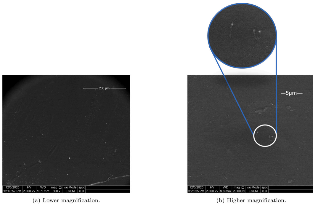
Fig. 7. SEM images of an epoxy sample reinforced with HNT (visible as dots and lines with diameter of approximately 30–70 nm and length of approximately 1–3 μm).
