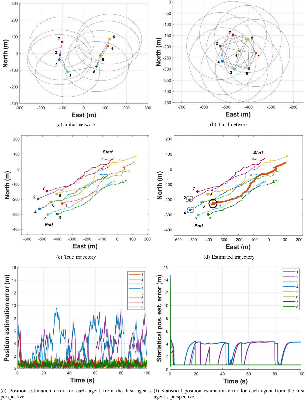
Fig. 4. Performance of flocking control with the distributed estimation under a time-varying network topology.
