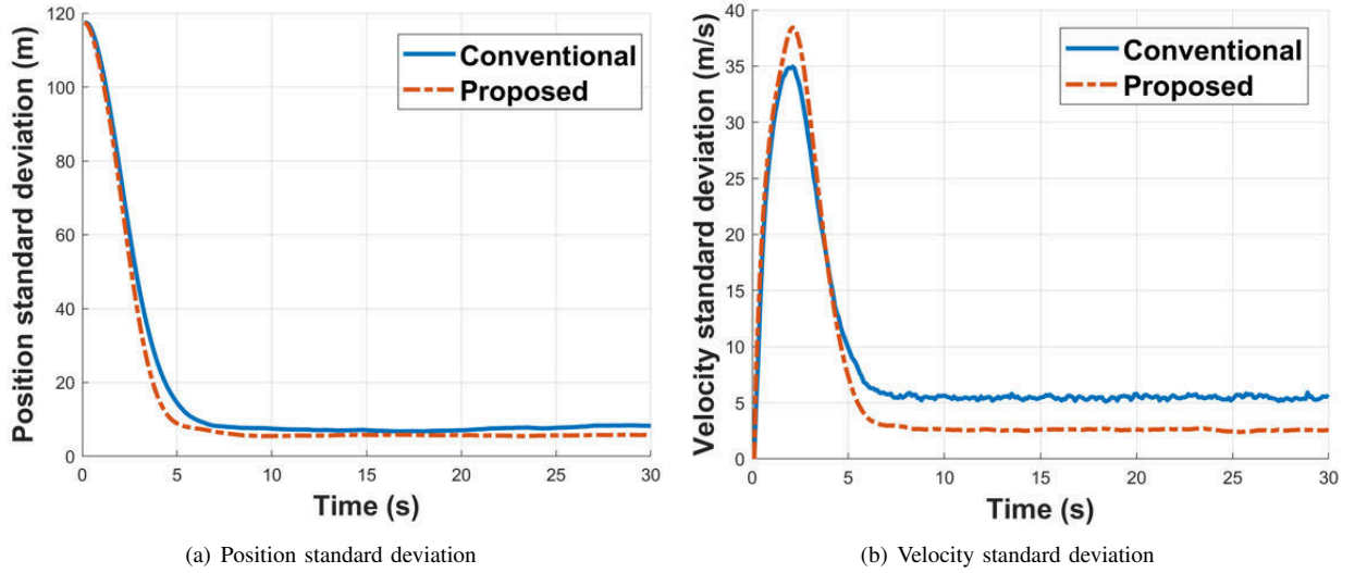
Fig. 3. Rendezvous control performance comparison.
