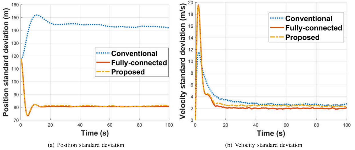
Fig. 5. Flocking control performance comparison.
