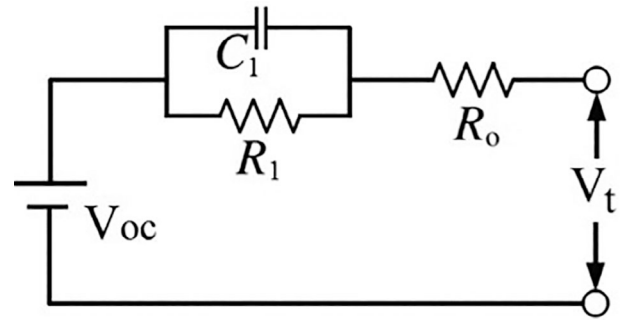
FIGURE 9 Battery electrical circuit model (Thevenin model)
