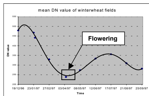
Figure 71. Typical evolution of ERS data over wheat fields, with the flowering date indicated.
