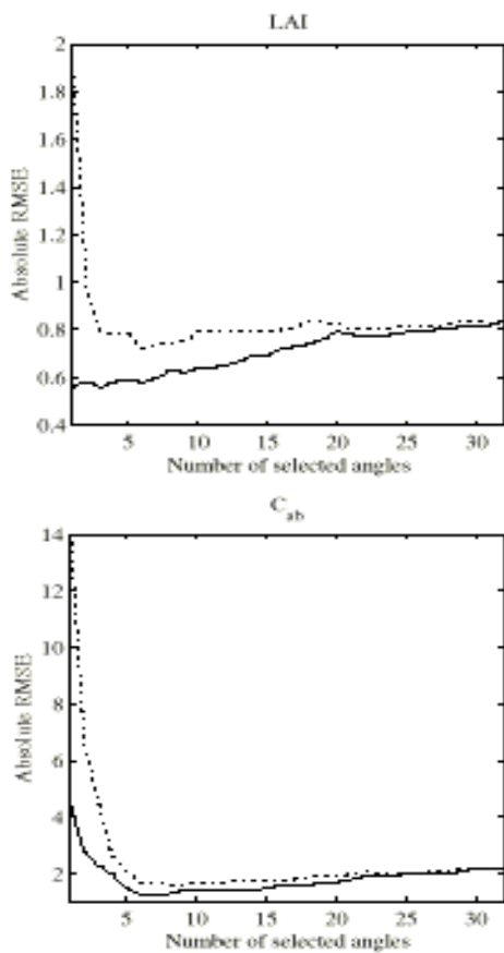
Figure 23 Absolute RMSE value between actual and estimated canopy variable ( LAI and Cab ) as a function of the number of selected directions. The solid line and the dashed line corresponds respectively to the best and worse sets of directions.
