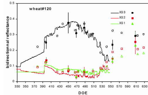
Figure 67. Comparison between our reflectance simulations (solid lines) based on STICS+SAIL to the actual ReSeDA POLDER (simple dots) and SPOT data (dots with vertical bars).
