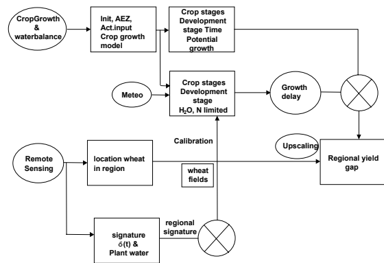
Figure 70. Combination methodology for the estimation of yield at the regional level using remote sensing and crop growth simulation. AEZ=Agro Ecological Zone, N=nitrogen.
