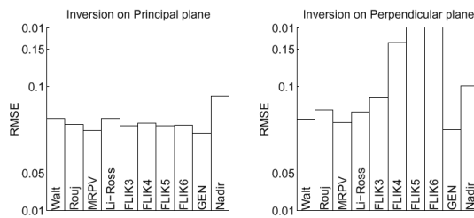
Figure 31. Extrapolation performances of the BRDF models. The models are adjusted either over the data close to principal plane (left) or close to the perpendicular plane (right). They are then tested over all the POLDER data.
