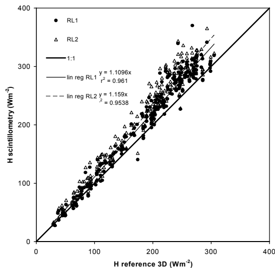
Figure 57. Comparison between spatially-averaged sensible heat flux derived from eddy correlation measurements and from scintillometry, using 2 aggregation schemes for roughness length.
