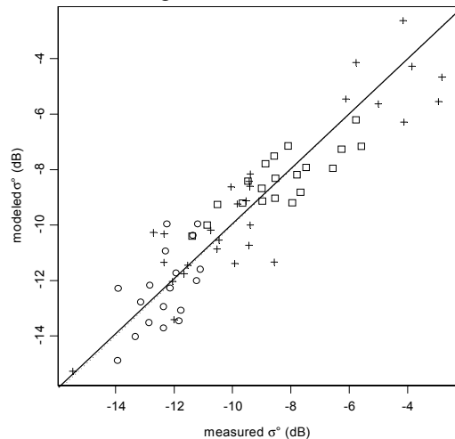
Figure 46 fitting the CLOUD model on ERASME data: modeled vs. measured \sigma^\circ . Data acquired at 20°: plus, at 40°: open squares. (a) C-HH, (b) C-VV, (c) X-HH, (d) X-VV. The solid line is the 1:1 line.
