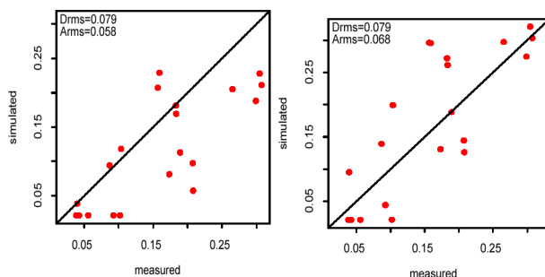
Figure 74. Comparison of measured top layer soil moisture values to those estimated by assimilation of POLDER and ERS and Radarsat data (left) and POLDER only (right) over field 300.
