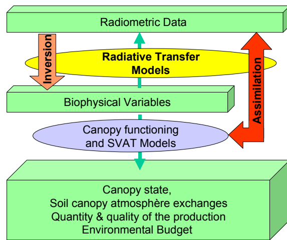
Figure 6. Flow chart diagram showing how to infer end variables such as canopy net primary production (NPP), yield or water fluxes from assimilation of remote sensing data into canopy and soil models. The inversion is restricted to the retrieval of canopy biophysical variables using radiative transfer models in the inverse mode. The green arrows indicate the way models work in the forward direction.
