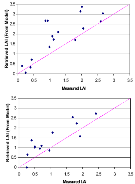
Figure 51. Comparison between measured LAI values of wheat (top) and sunflower (bottom) and those estimated from a semi-empirical polynomial model.
