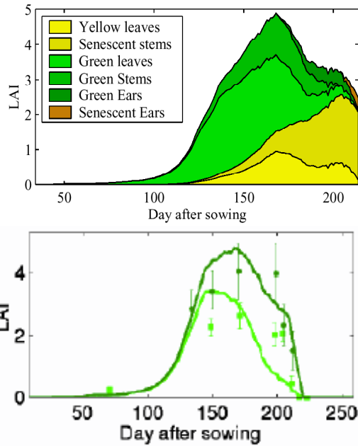
Figure 66. Simulation of the OAI for a wheat field in ReSeDA (top). The bottom graph shows the dynamics of the green LAI as measured by planimetry (dots) or simulated by our STICS adaptation (light green). Total green OAI is also compared to the LAI2000 measurements (dark green).
