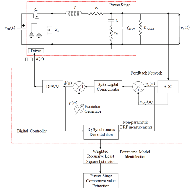
Fig. 9. Modified Block Diagram of Parametric Identification Based Health-Monitoring on Digitally-Controlled DC-DC Buck Converter for Aging Detection on Power-Stage Network Elements
