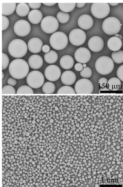
Fig. 6. SEM images of the MIP particles ( D_{v,0.5}^p = 141 \mu\text{m} , span = 0.96) taken at different magnifications. The emulsion was prepared at 400 rpm, J_d = 200 \text{Lm}^{-2}\text{h}^{-1} , and \phi_o = 23 vol%.
