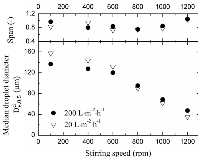
Fig. 4. The effect of stirring rate during membrane emulsification on the volume median diameter, D_{V,0.5}^d , and the span at J_d = 20 and 200 \text{ L}\cdot\text{m}^{-2}\cdot\text{h}^{-1} . The dispersed (oil) phase content \phi_o at the end of the emulsification process was 9 vol%.
