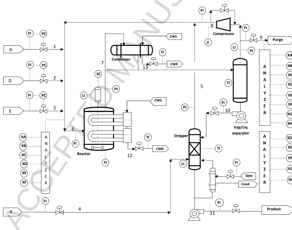
Figure 1 Graphical Description of the TEP Plant
