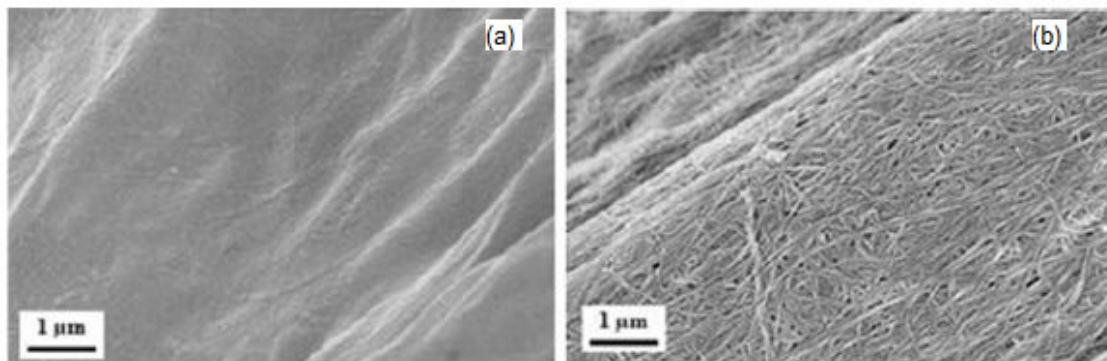
Fig. 9 SEM micrographs (a) sisal fiber and (b) bacterial cellulose coated sisal fiber [61]
