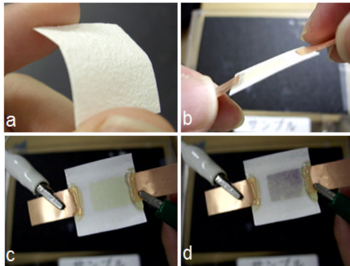
Fig. 19 a) the paper made of nanocellulose; b) display device; c) and d) show the result of the Chromogenic testing [188]
