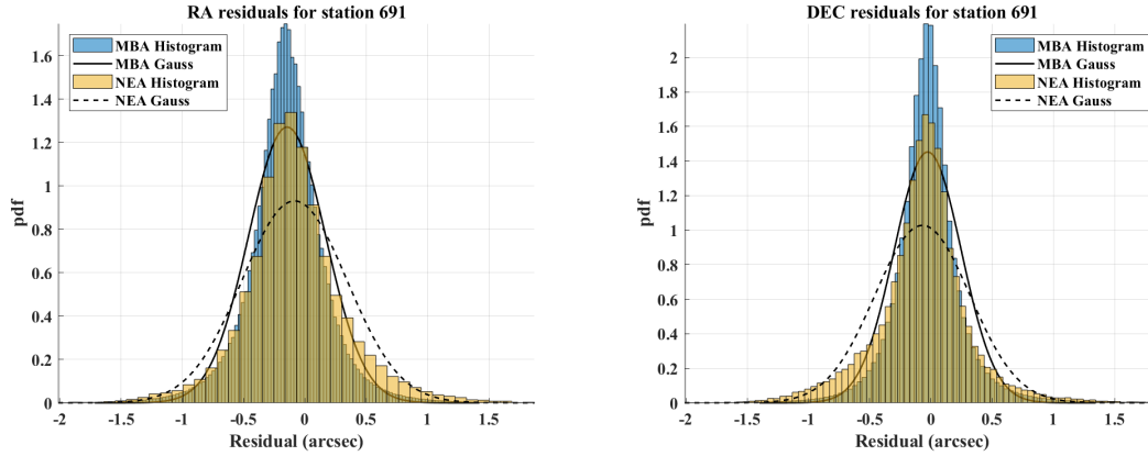
Fig. 2: Probability density function (pdf) of the distribution of the residuals for station 691 in Right Ascension (left panel) and Declination (right panel). The histogram and the Gaussian Normal Distribution are represented superimposed for the residuals of MBA and NEA observations distinctly.
