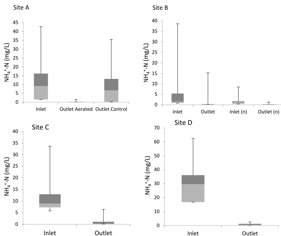
Figure 3. Box and whisker plot of \text{NH}_4^+\text{-N} concentrations at the inlet and the outlet of the control and aerated beds. ( n = Site B data excluding the upstream process failure). The box represents the interquartile range; the line indicates the mean and the whiskers the 25th and 75th percentiles.
