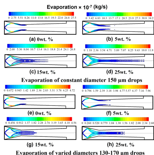
Figure 12. Evaporation rates of drops inside the domain for group injection with a constant diameter of (a–d) 150 \mu\text{m} and with varied diameters of (e–h) 130–170 \mu\text{m} , having 0, 5, 15, and 25 wt % nanoparticle concentrations.
