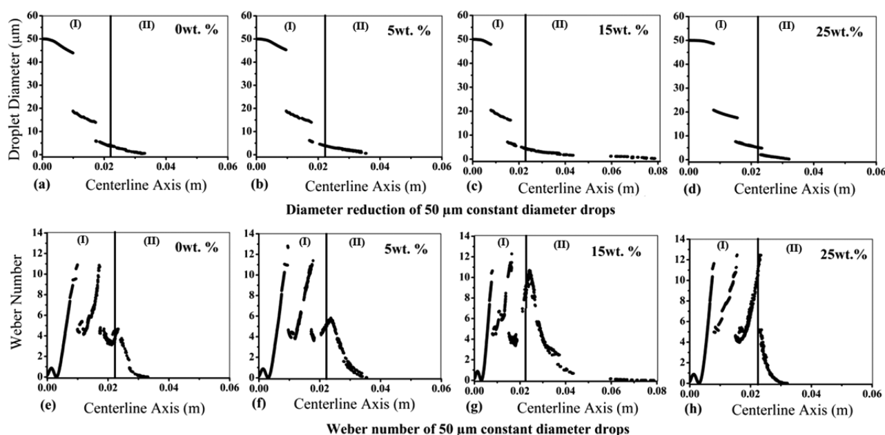
Figure 7. Comparison of (a–d) droplet diameter reduction and (e–h) Weber number for surface-type injection with a constant diameter of 50\ \mu\text{m} having 0, 5, 15, and 25 wt % nanoparticle concentrations.
