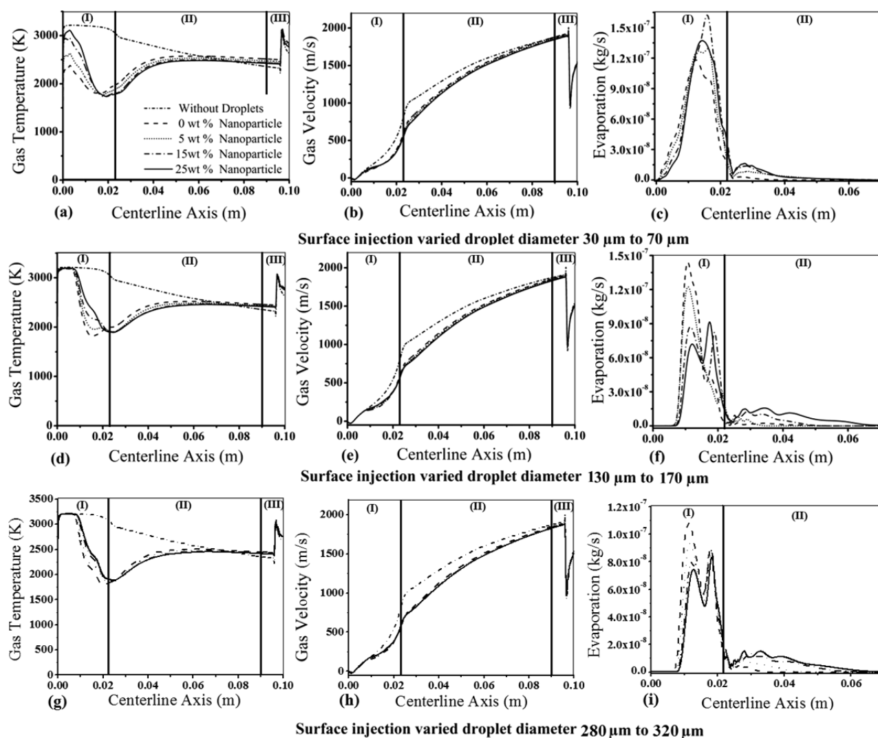
Figure 4. Comparison of gas temperature, gas velocity field, and rate of evaporation experienced by droplets injected from the surface with varied diameters of (a–c) 30, 40, 50, 60, and 70 \mu\text{m} ; (d–f) 130, 140, 150, 160, and 170 \mu\text{m} ; and (g–i) 280, 290, 300, 310, and 320 \mu\text{m} , having different solid nanoparticle concentrations.
