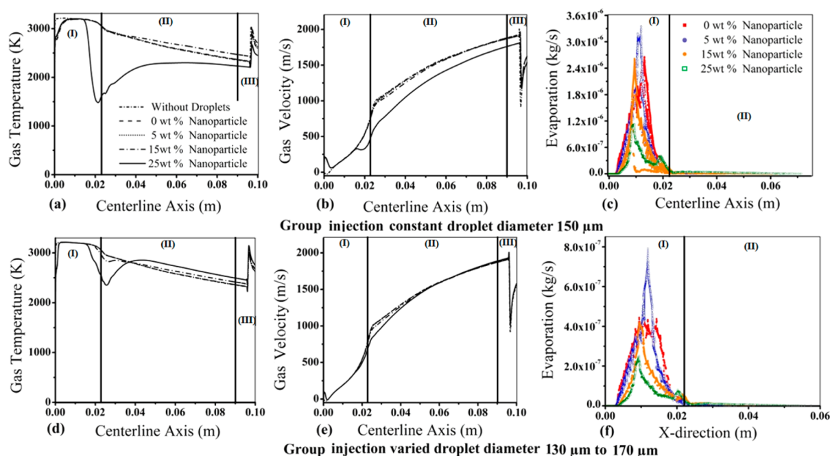
Figure 6. Comparison of gas temperature, gas velocity field, and rate of evaporation experienced by droplets injected as a group at an angle of injection of 45^\circ with constant diameter (a–c) 150\ \mu\text{m} and with varied diameters of (d–f) 130, 140, 150, 160, and 170\ \mu\text{m} , having 0, 5, 15, and 25 wt % nanoparticle concentrations.
