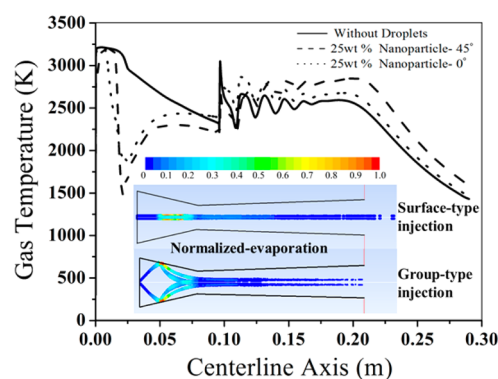
Figure 5. Comparison of gas temperature and normalized droplet evaporation with surface-type injection (angle of injection 0^\circ ) and group-type injection (angle of injection 45^\circ ) of constant diameter droplet of 150 \mu\text{m} and having 25 wt % nanoparticle concentrations.
