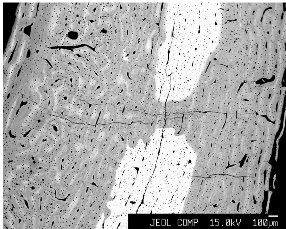
Fig. 10. Contrast differences due to burning of a 6-month decayed bone sample (WSF5D6M1_burnt). Note the central mineralised areas. (Electron microprobe, backscatter electron detector image.)
