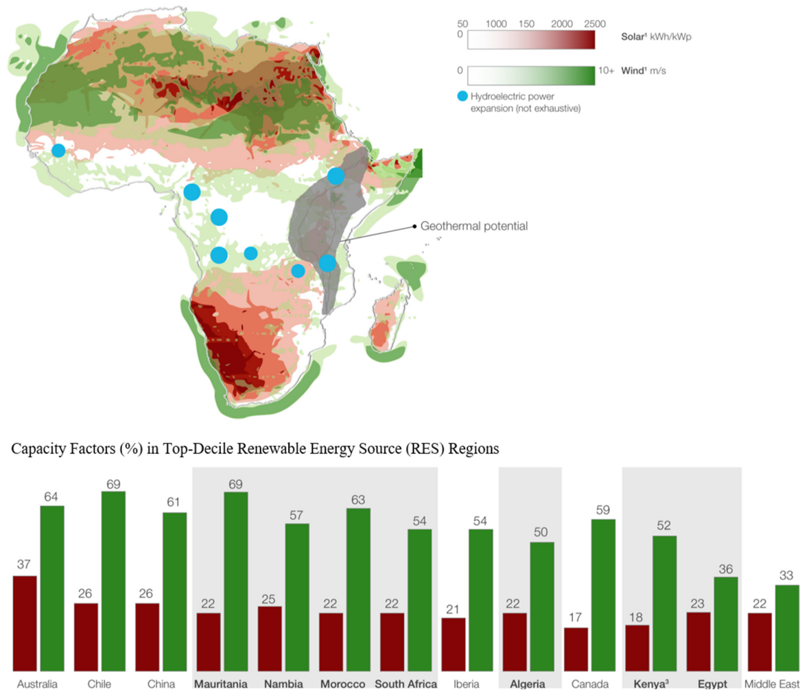
Figure 3. Map of renewable energy potential. 1. Solar energy potential (in kWh/kWp) and wind energy potential at 100 m above ground level (m/s). 2. Ranking of countries based on a 50:50 weighted average of capacity factors for the top 10% solar power [34,43].
