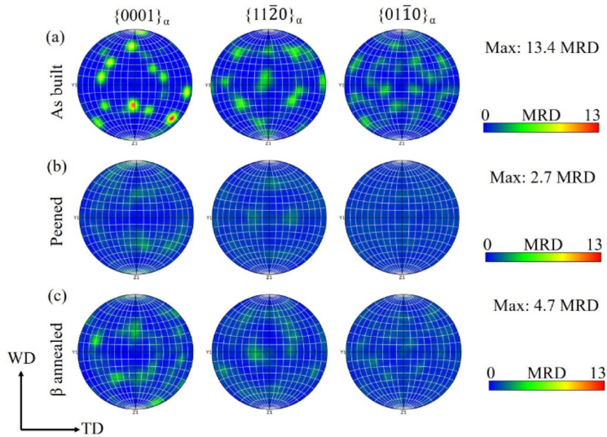
Fig. 3. Pole figures of \alpha phase measured in these conditions: (a) as-built, (b) peened, (c) peened + \beta annealed.
