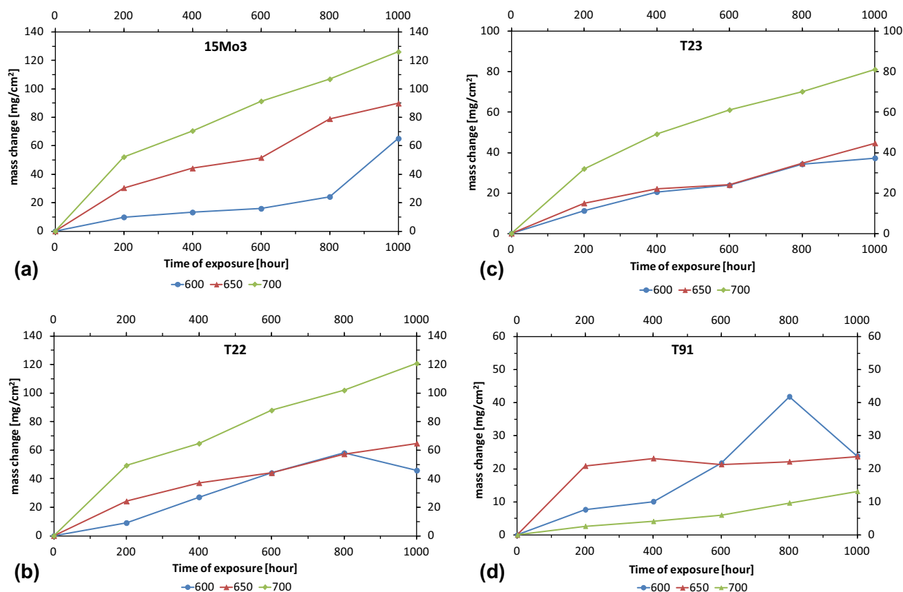
Fig. 3 Mass change vs. exposure time for (a) 15Mo3, (b) T22, (c) T23 and (d) T91 at 600, 650 and 700 °C under fireside atmosphere for 1000 h
