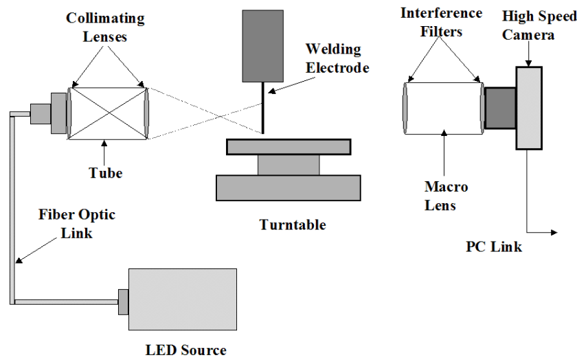
Fig 1. High-speed camera and LED backlighting configuration
