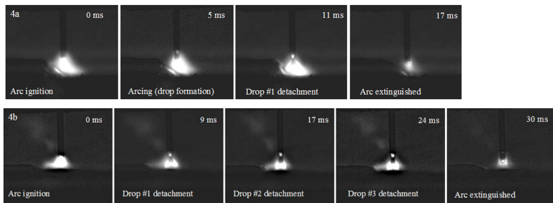
Fig 4. Arcing phase droplet detachment. a. Wf 5.5 \text{ m min}^{-1} , 1 droplet. b. Wf 6 \text{ m min}^{-1} , 3 droplets
