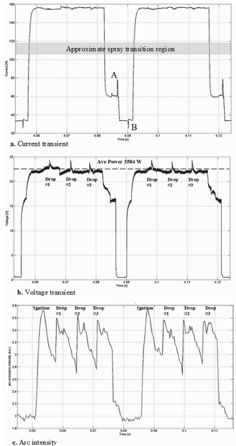
Fig. 5. CMT transients ( Wf\ 6\text{m min}^{-1} ) a. Current trace; b. Voltage trace; c. Arc plasma intensity (arbitrary values)
