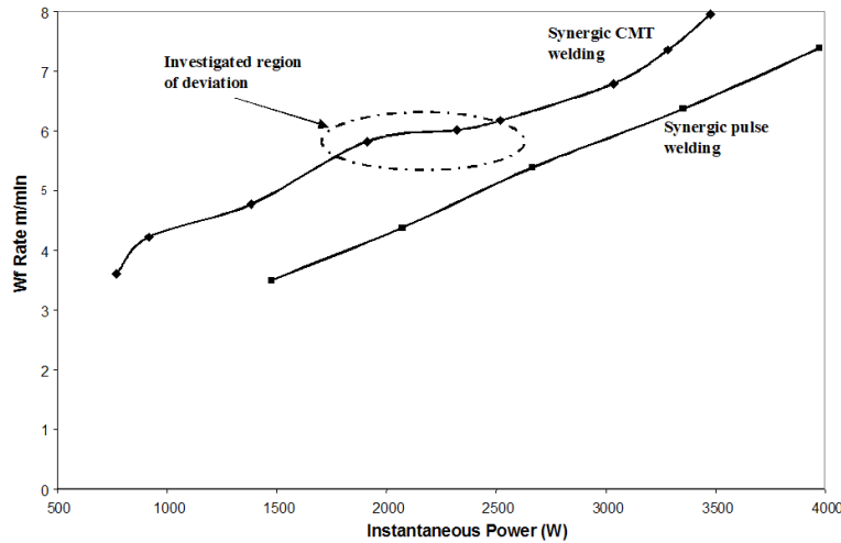
Fig 3. Comparative deposition – synergic CMT v Pulse welding using 1.2mm Al-4043 filler
