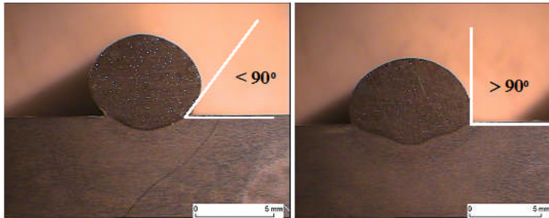
Fig 7. Weld contact angle definition
