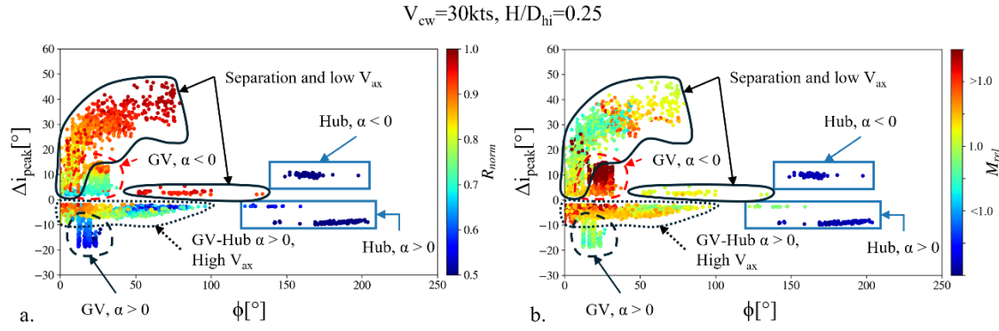
Figure 11 Peak swirl distortion events tracked for the fan blades for H/D_{hi}=0.25 , V_{cw}=30 kts, coloured by (a.) R_{norm} and (b.) M_{rel} .
