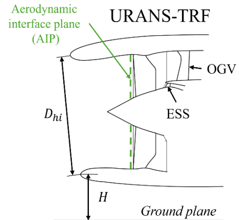
Figure 1 Schematic representation of intake-fan configuration.
