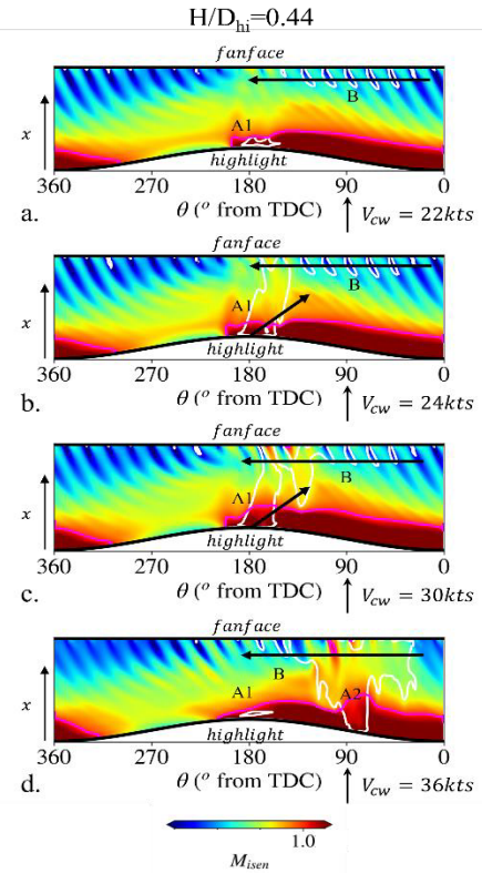
Figure 6 Snapshot of M_{isen} on the unwrapped intake surface with isoline of M_{isen}=1 (magenta), and axial wall shear stresses \tau_{wx}=0 (white) for H/D_{hi}=0.44 at (a.) V_{cw}=22\text{kts} , (b.) V_{cw}=24\text{kts} , (c.) V_{cw}=30\text{kts} , (d.) V_{cw}=36\text{kts} .
