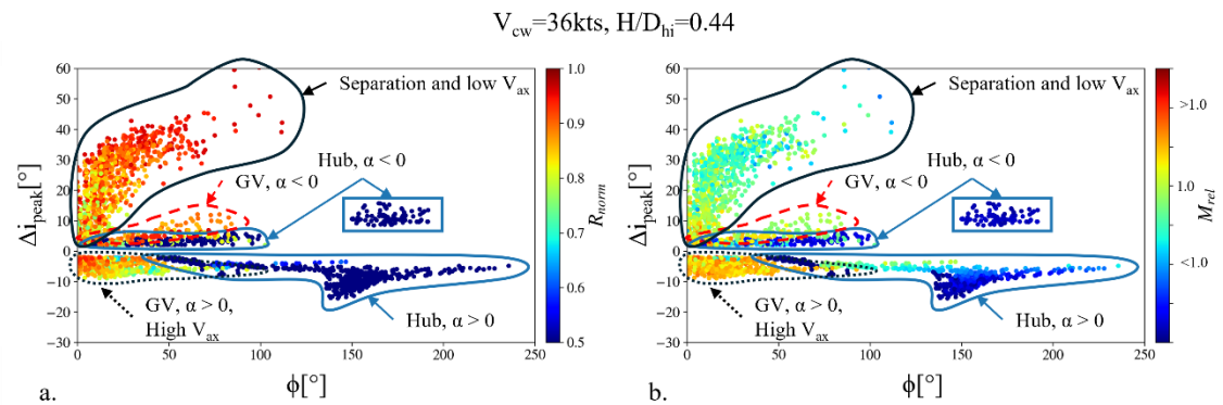
Figure 13 Peak swirl distortion events tracked for the fan blades for H/D_{hi}=0.44 , V_{cw}=36 kts, coloured by (a.) R_{norm} and (b.) M_{rel} .
