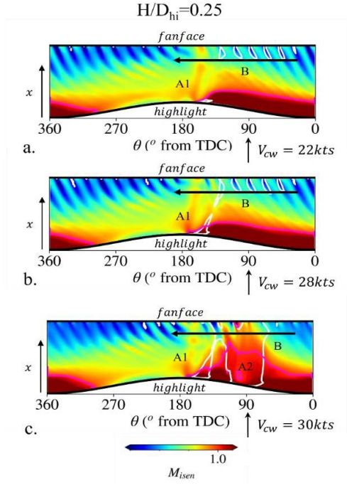
Figure 4 Snapshot of M_{isen} on the unwrapped intake surface with isoline of M_{isen}=1 (magenta), and axial wall shear stresses \tau_{wx}=0 (white) for H/D_{hi}=0.25 at (a.) V_{cw}=22\text{kts} , (b.) V_{cw}=28\text{kts} , (c.) V_{cw}=30\text{kts} .
