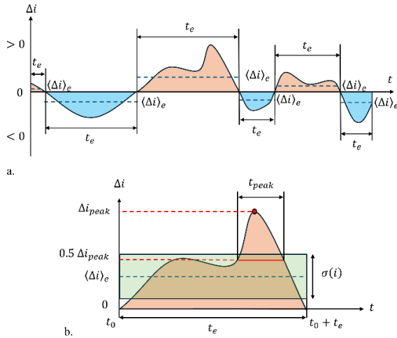
Figure 2 (a.) Time variation of \Delta i and blade distortion events; (b.) peak distortion event (based on [26]).
