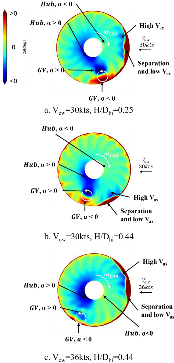
Figure 9 Snapshot of \Delta i for (a.) H/D_{hi}=0.25 , V_{cw}=30kts , (b.) H/D_{hi}=0.44 , V_{cw}=30kts , (c.) H/D_{hi}=0.44 , V_{cw}=36kts .
