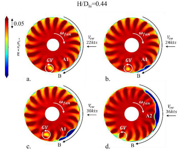
Figure 5 Snapshot of intake total pressure ratio for H/D_{hi}=0.44 at a. V_{cw}=22\text{kts} , b. V_{cw}=24\text{kts} , c. V_{cw}=30\text{kts} , d. V_{cw}=36\text{kts} .
