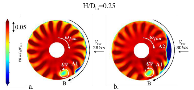
Figure 3 Snapshot of intake total pressure ratio for (a.) V_{cw}=28 kts, H/D_{hi}=0.25 , (b.) V_{cw}=30 kts, H/D_{hi}=0.25 .
