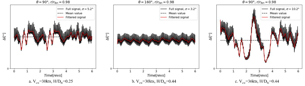
Figure 10 Time variation of \Delta i for (a.) H/D_{hi}=0.25 , V_{cw}=30\text{kts} , (b.) H/D_{hi}=0.44 , V_{cw}=30\text{kts} , (c.) H/D_{hi}=0.44 , V_{cw}=36\text{kts} .
