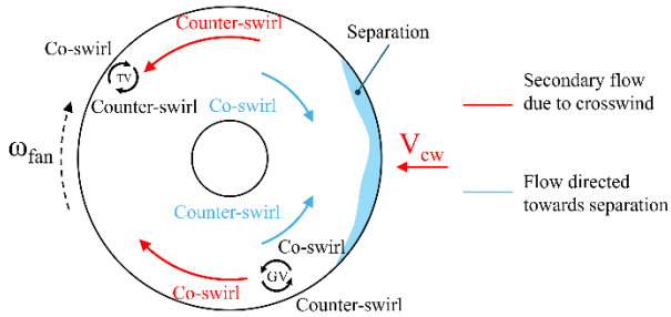
Figure 7 Secondary flows and vortices for an intake in crosswind for a counter-rotating configuration. Partially based on [13].
