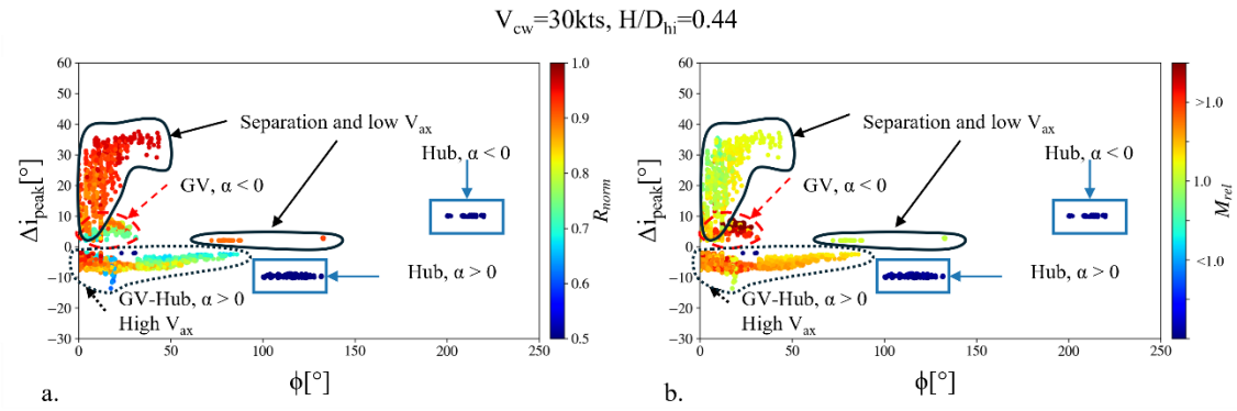
Figure 12 Peak swirl distortion events tracked for the fan blades for H/D_{hi}=0.44 , V_{cw}=30 kts, coloured by (a.) R_{norm} and (b.) M_{rel} .
