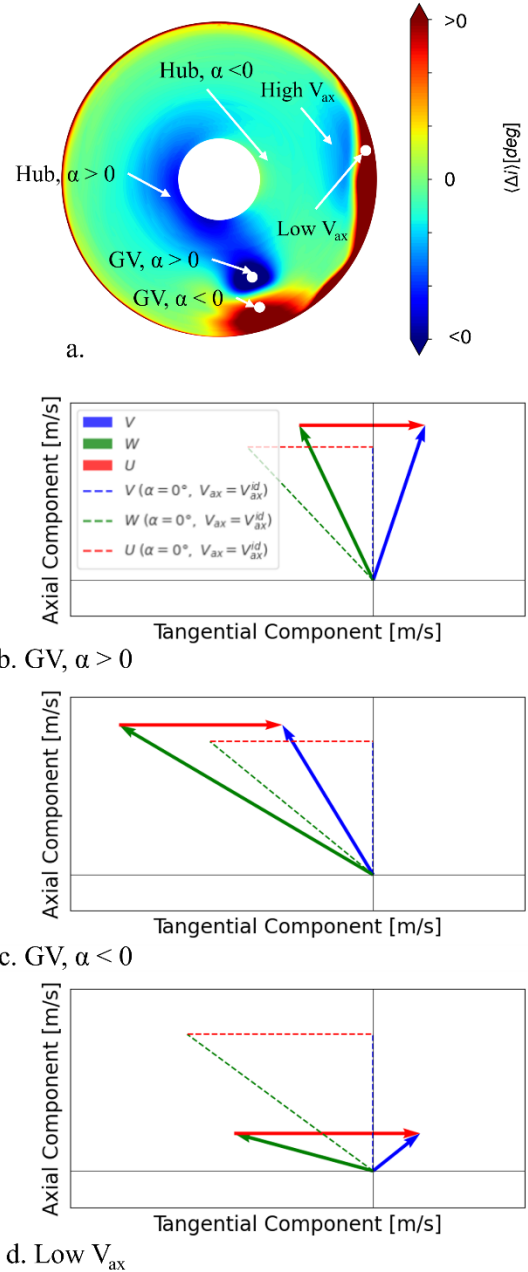
Figure 8 (a). Time-averaged distribution of \Delta i for H/D_{hi}=0.25 and V_{cw}=30 kts, time-averaged velocity triangles: (b) for the region of the GV with \alpha > 0 , (c) for the region of the GV with \alpha < 0 , (d) for the region at the tip with low V_{ax} .
