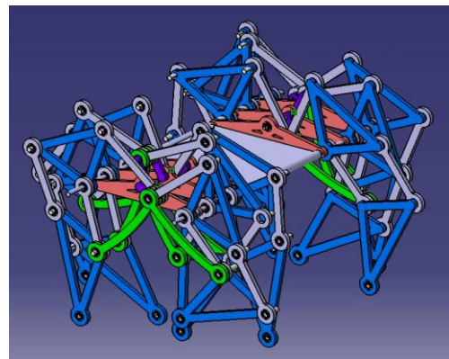
Figure 5 Full Jansen mechanism locomotion assembly model for WANDER-Bot
