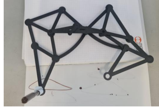
Figure 3 Experimental Jansen mechanism walking gait
