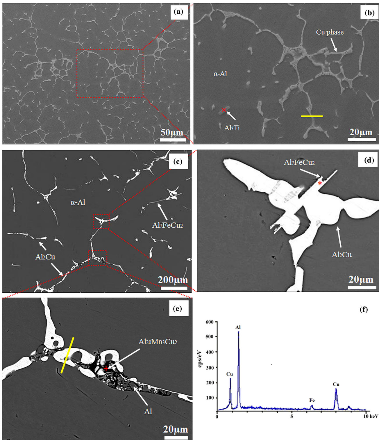
Fig. 6—Microstructures and EDX analysis of the 201 alloy: (a) as-received, (b) high-magnification micrograph showing grain boundaries and Al 3 Ti particles, (c) after DSC test (d) high-magnification micrograph showing the Al 7 FeCu 2 particle, (e) high-magnification micrograph showing the Al 20 Mn 3 Cu 2 particle, (f) EDX spectrum for Al 7 FeCu 2 phase, marked as asterisk in (d), (g) EDX spectrum for Al 20 Mn 3 Cu 2 phase, marked as plus symbol in (e), (h) EDX spectrum for Al 3 Ti phase, marked as multiply symbol in (b), (i) line analysis across a grain boundary in (b), (j) line analysis across a grain boundary in (e).
