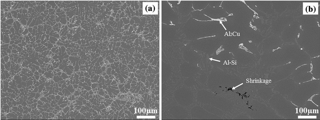
Fig. 4—SEM back scattered images of the 319s alloy: (a) as MHD processed, (b) after DSC test (3 K/min with ~20 mg sample).
